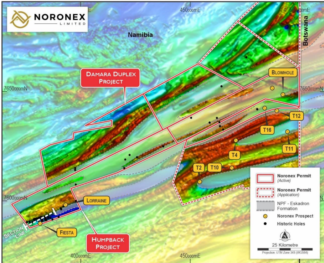
Figure 2: Regional aeromagnetic image of the Kalahari Copper Belt in Namibia with the current Noronex projects showing Fiesta in the west and Blowhole in the east
