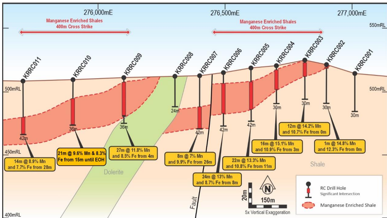
Figure 3. KR1 cross-section 7,475,100mN (looking to the north) with manganese enriched shale and drill intersections.
