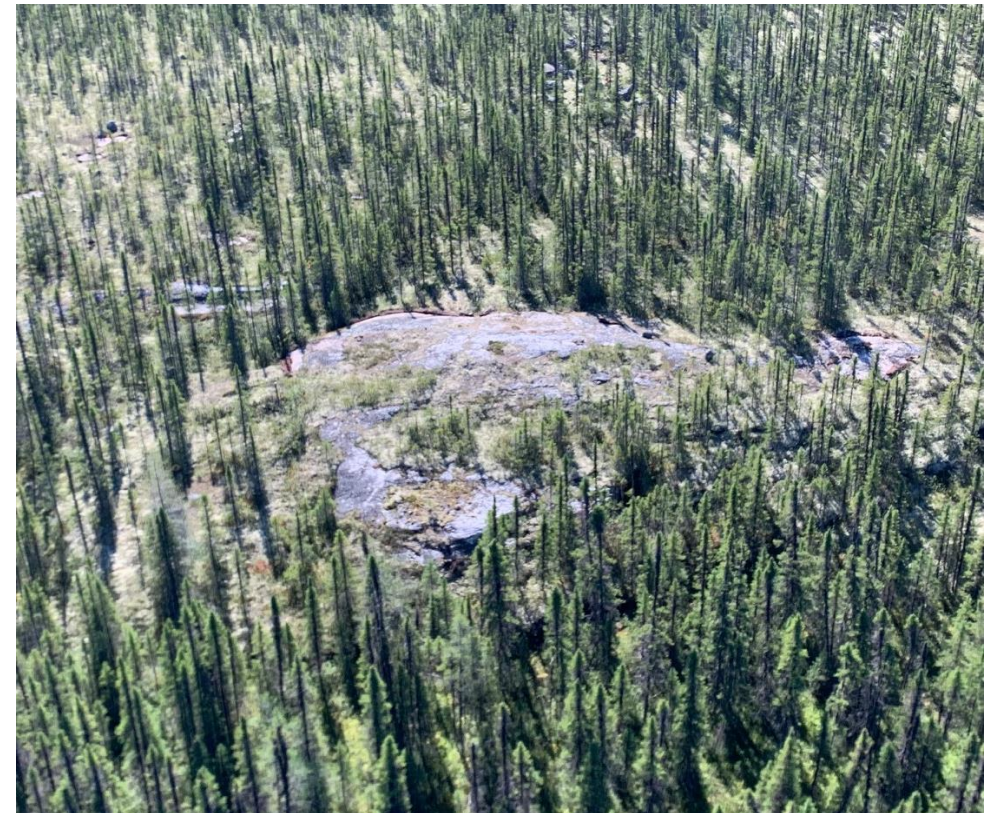
Figure 1.7 Discovery outcrop - Adina Main Zone
