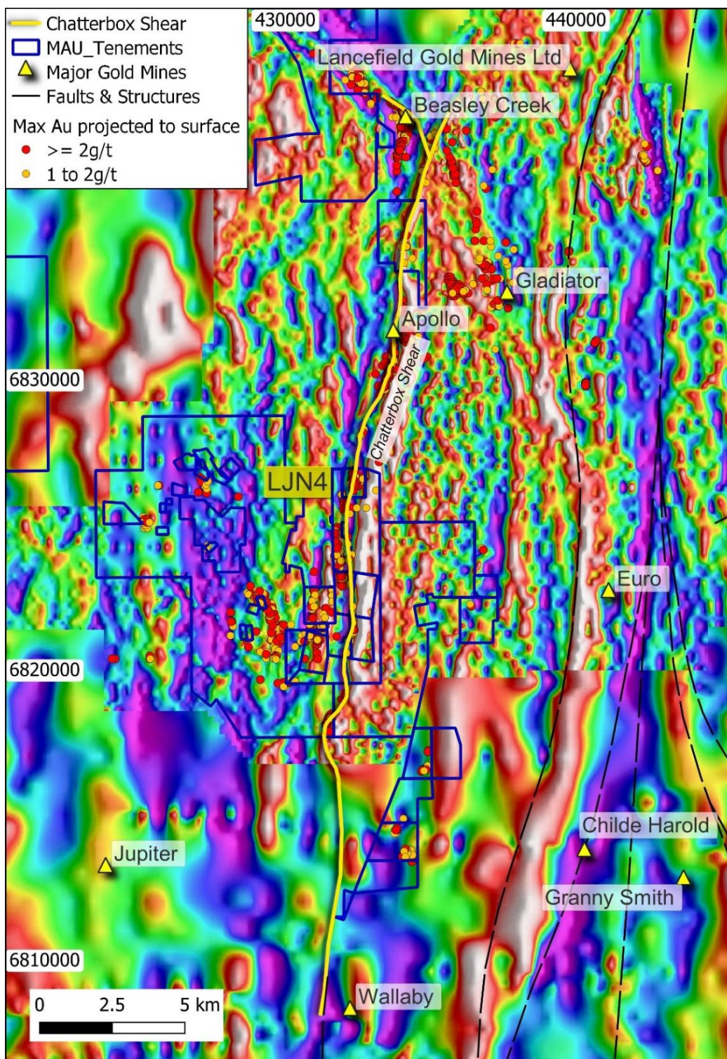
Figure 4. The Lady Julie North 4 Chatterbox Interpreted Shear shown on a Gravity image with major gold deposits.
