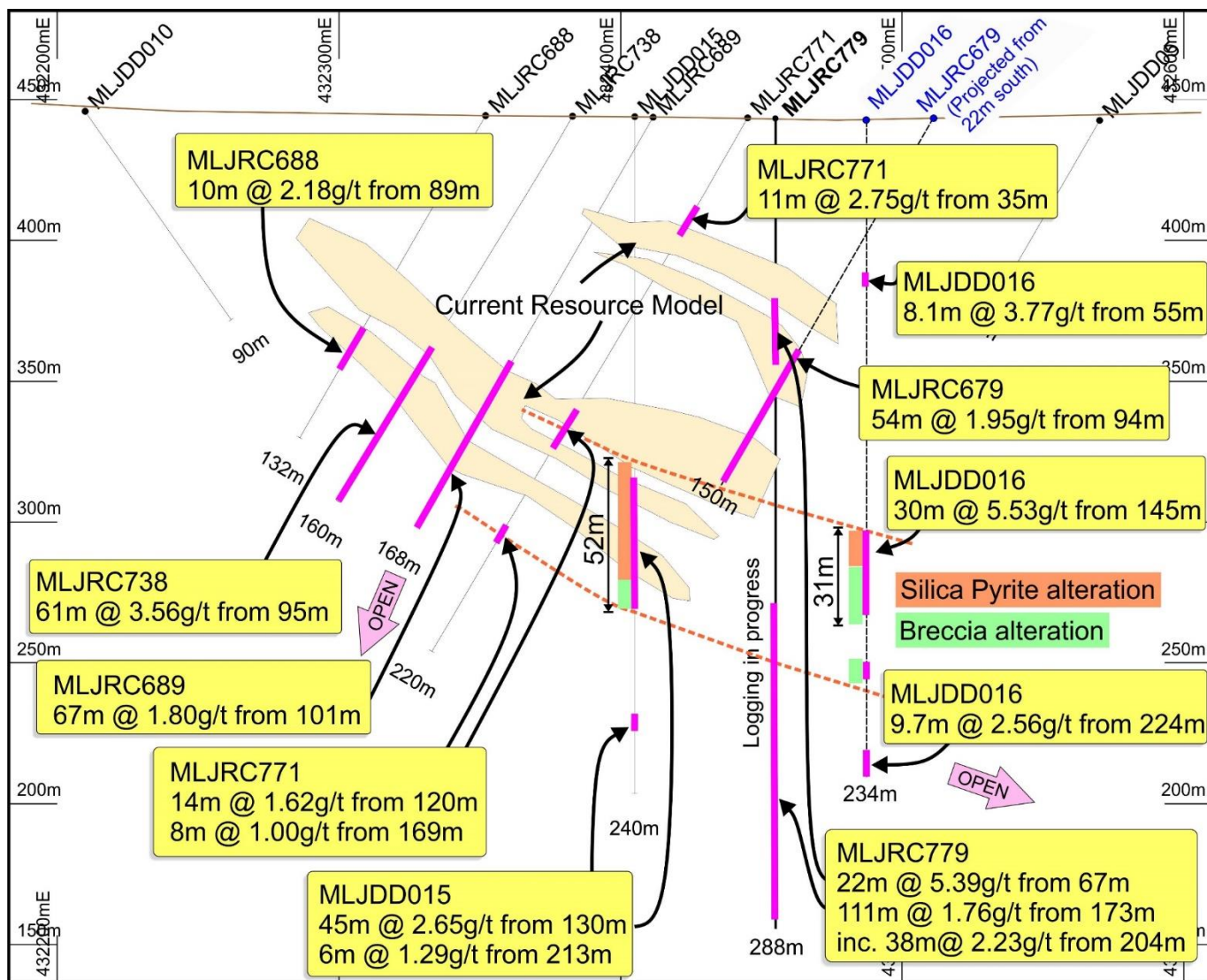
Figure 2. Composite cross section for LJV4 centre area showing thickened high-grade dipping gold zone containing breccia and silica-pyrite alteration, upper mineralised zone, older resource model outline, thickened mineralisation in drill hole MLJRC779 and potential depth extensions at depth, downdip to the east and south.
