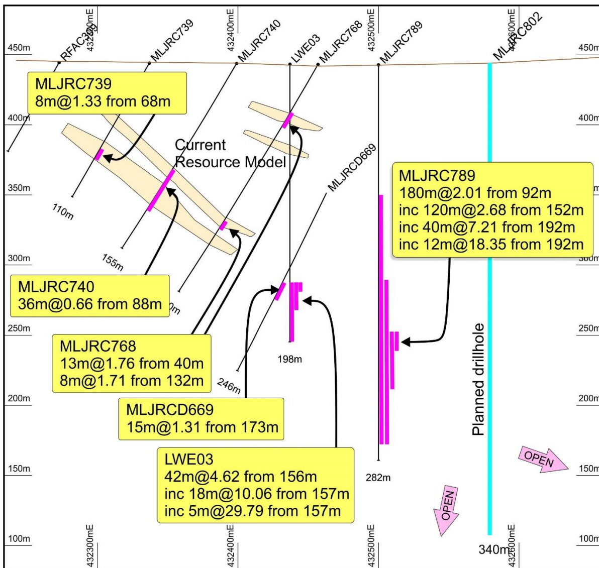
Figure 1. Cross section for LJA4 centre area showing thickened high-grade dipping gold zone containing, upper mineralised zone, older resource model outline, new drill hole MLJRC789 and potential depth extensions at depth, downdip to the east and at depth.
