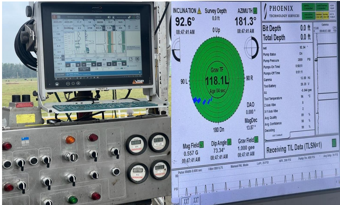
Figure 3. Ensign Rig 438 control panels used for rig management and directional drilling.
