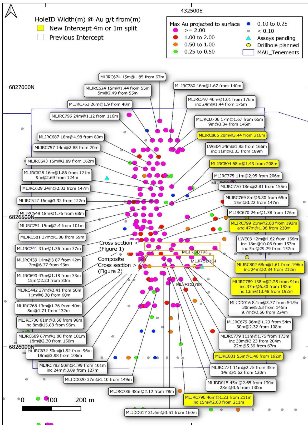
Figure 3. The Lady Julie North 4 deposit has numerous significant thick intersections from the latest drill programme (yellow large rectangular label) and previous drilling (white label) with maximum gold projected to surface and planned deeper drillholes (in yellow) and holes with assays awaited (in blue).
