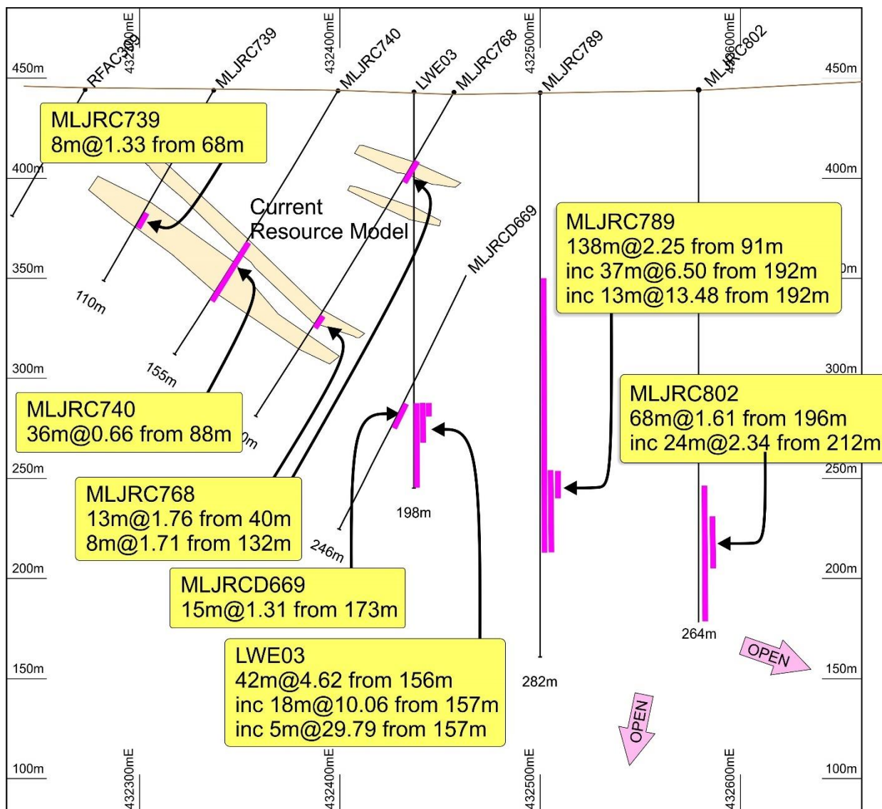
Figure 1. Cross section for LJV4 centre area showing thickened high-grade dipping gold zone containing, upper mineralised zone, older resource model outline, new drill hole MLJRC802 and potential depth extensions at depth, downdip to the east and at depth.
