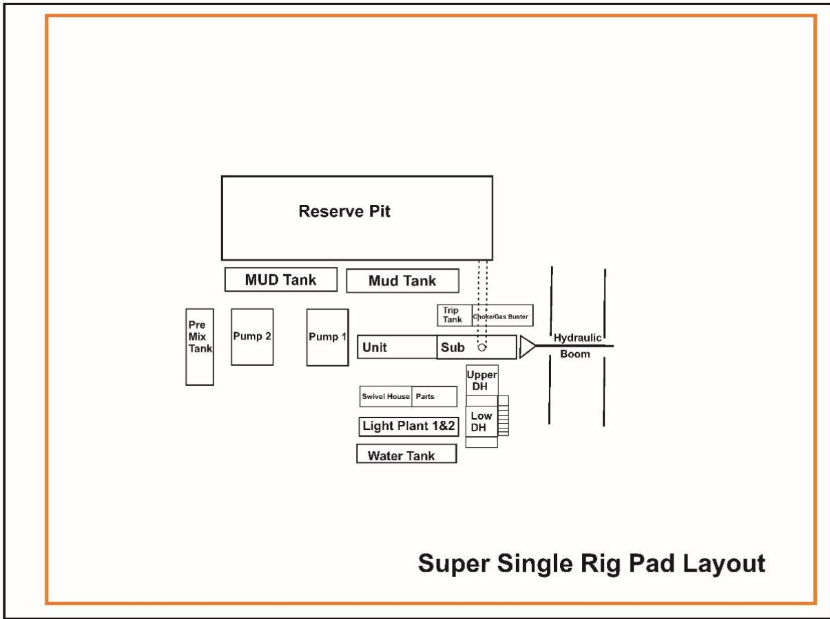
Figure 3: The small pad layout required to drill the wells on the recently purchased private property.
