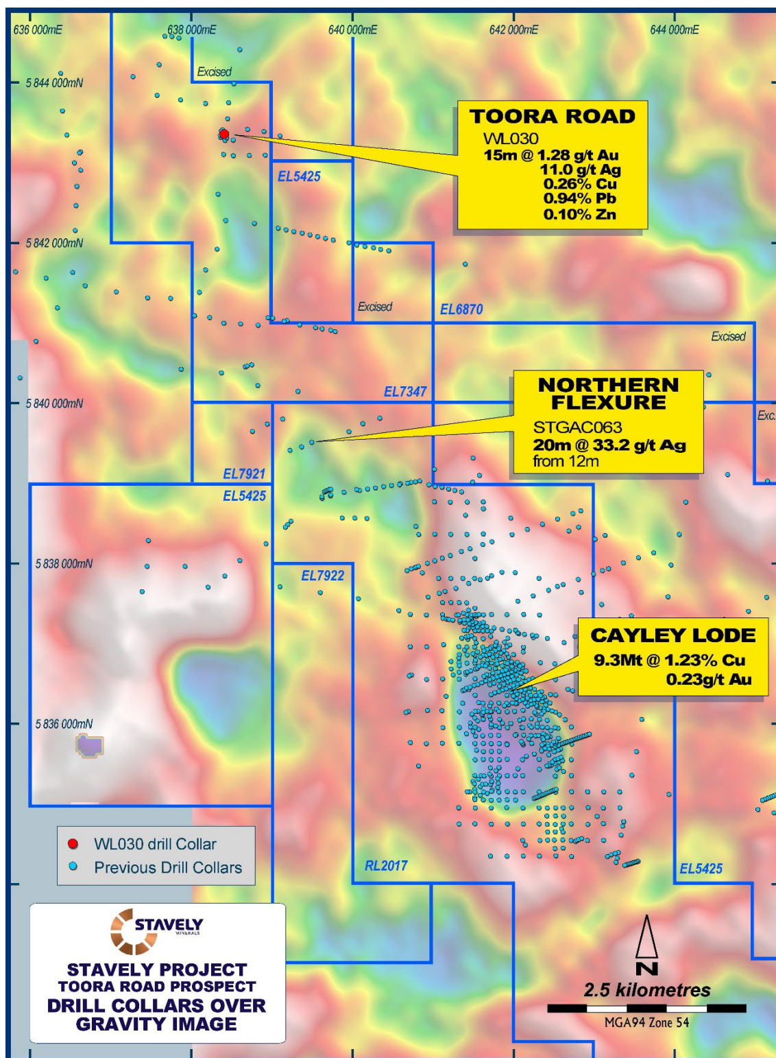
Figure 6. Thursday's Gossan (Cayley Lode), Northern Flexure and Toora Road prospects are associated with distinct gravity lows interpreted to be related to hydrothermal clay alteration which is less dense than the unaltered host rocks.
