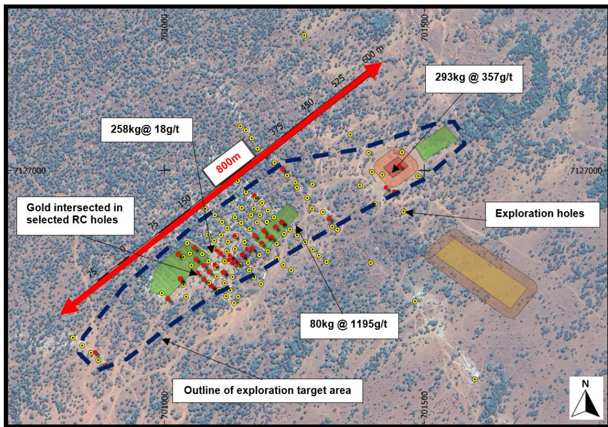
Figure 3: Exploration Target resource area at Revere Project
