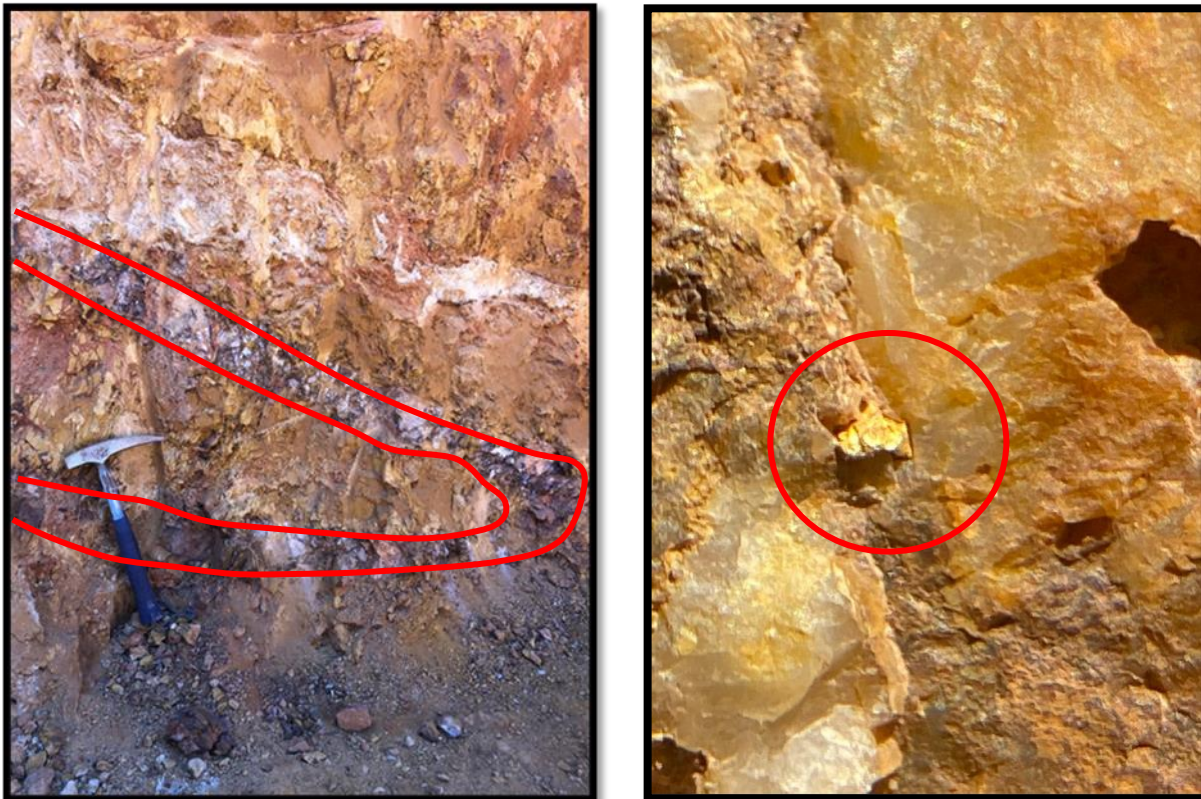
Figure 2: Visible gold in the Revere Reef system (coasten location: 701112.71, N7126828)
