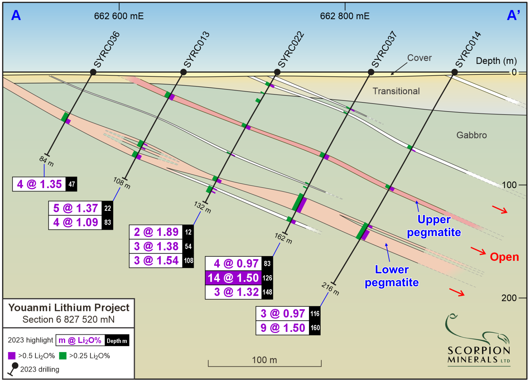
Figure 3: Section A-A' 6 827 520 mN
