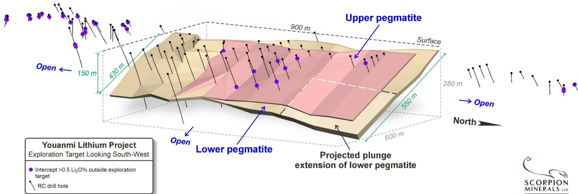
Figure 4: Oblique view of Exploration Target looking Southwest
