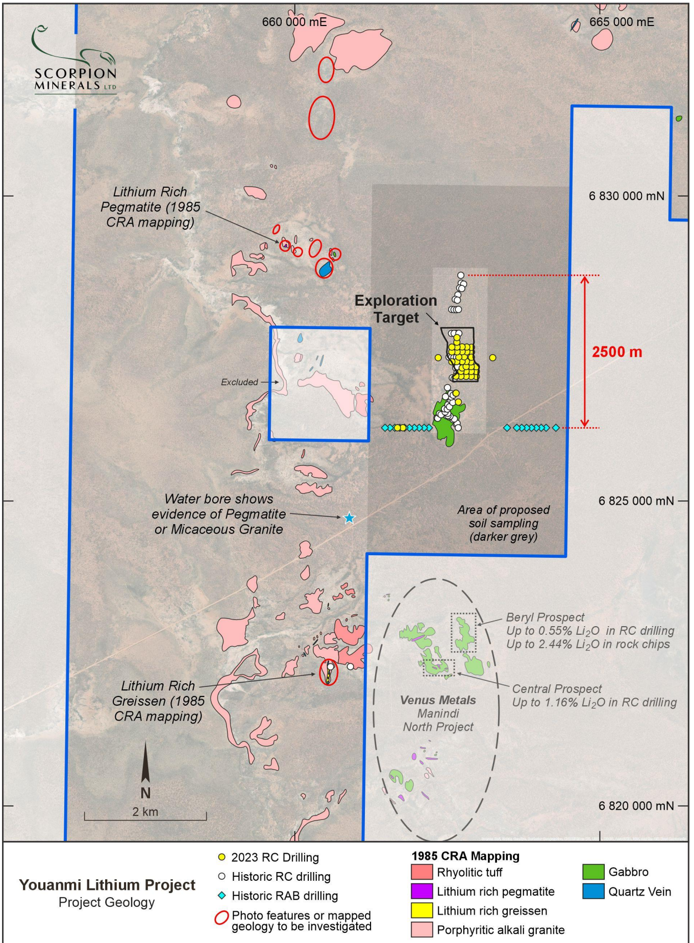
Figure 5: Local Outcrop Geology
