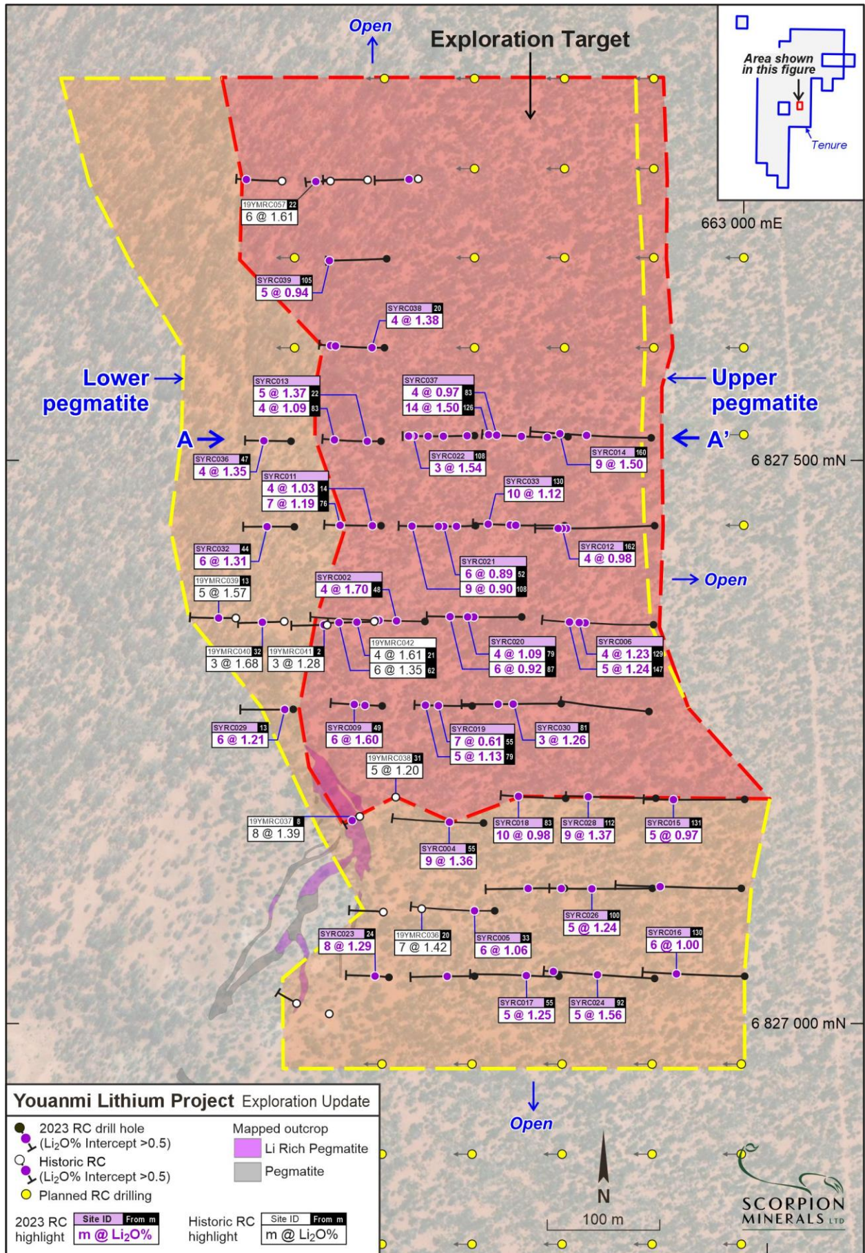
Figure 2: Plan enlargement showing mapped pegmatite outcrop and significant RC Drilling intercepts.
