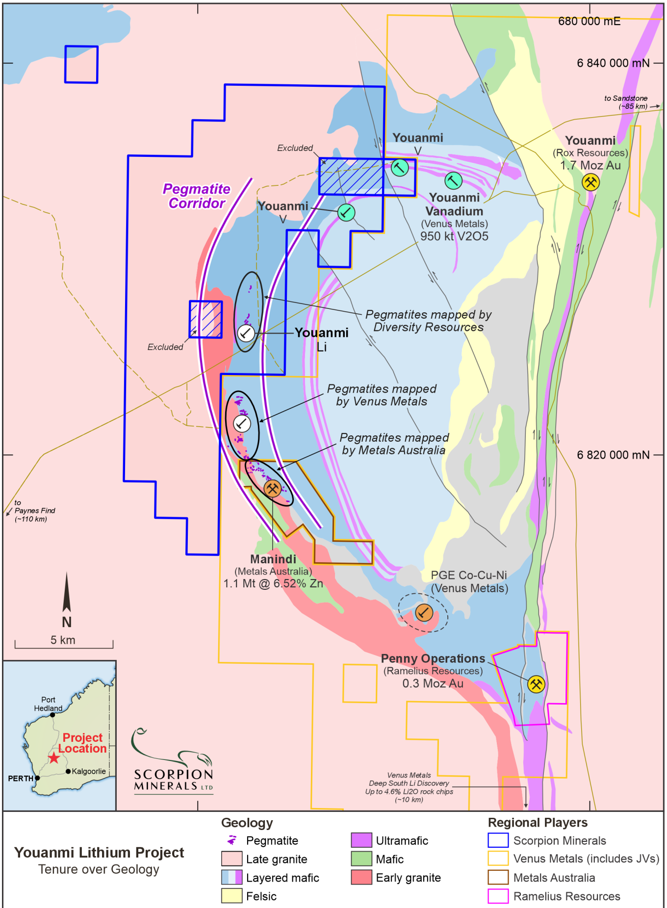
Figure 6: Plan Showing Tenements over Simplified Regional Geology and Adjacent Explorers
