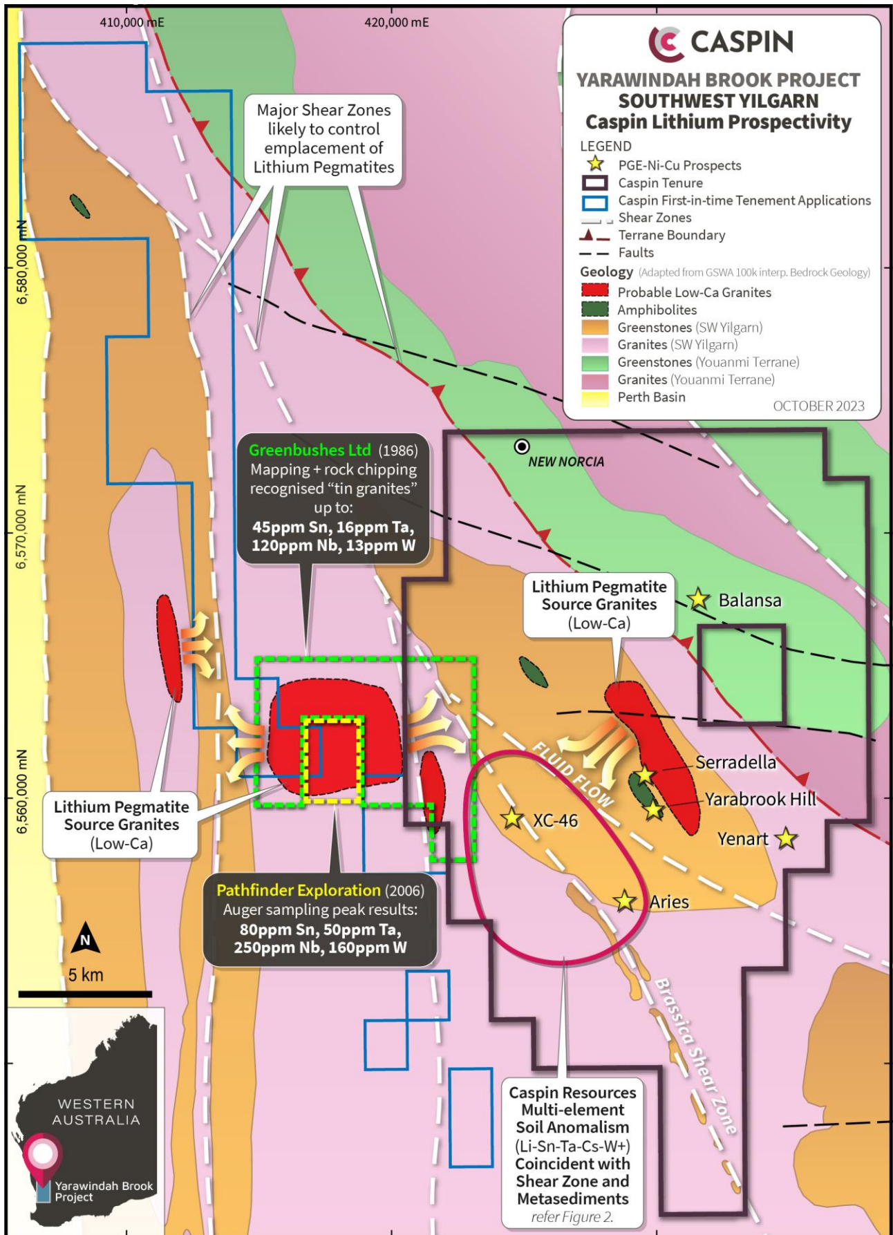
Figure 1. Conceptual lithium mineralisation model, structural and stratigraphic setting of Yarawindah Brook.
