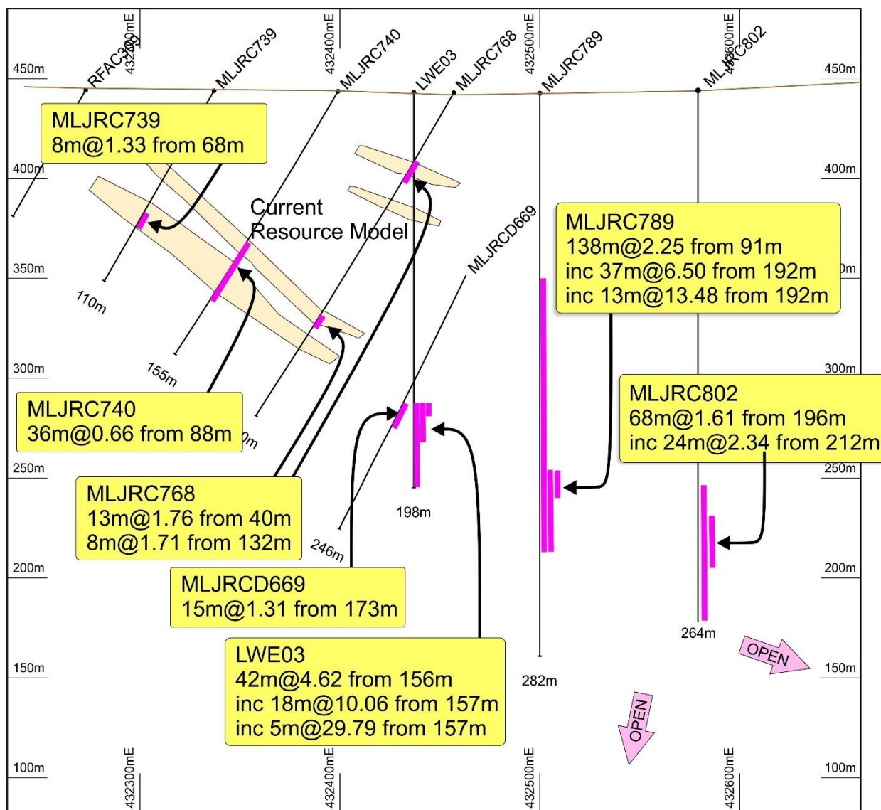
Figure 1. Cross section for LJN4 centre area showing thickened high-grade dipping gold zone containing, upper mineralised zone, older resource model outline, new drill hole MLJRC802 and potential depth extensions downdip to the east and at depth.
