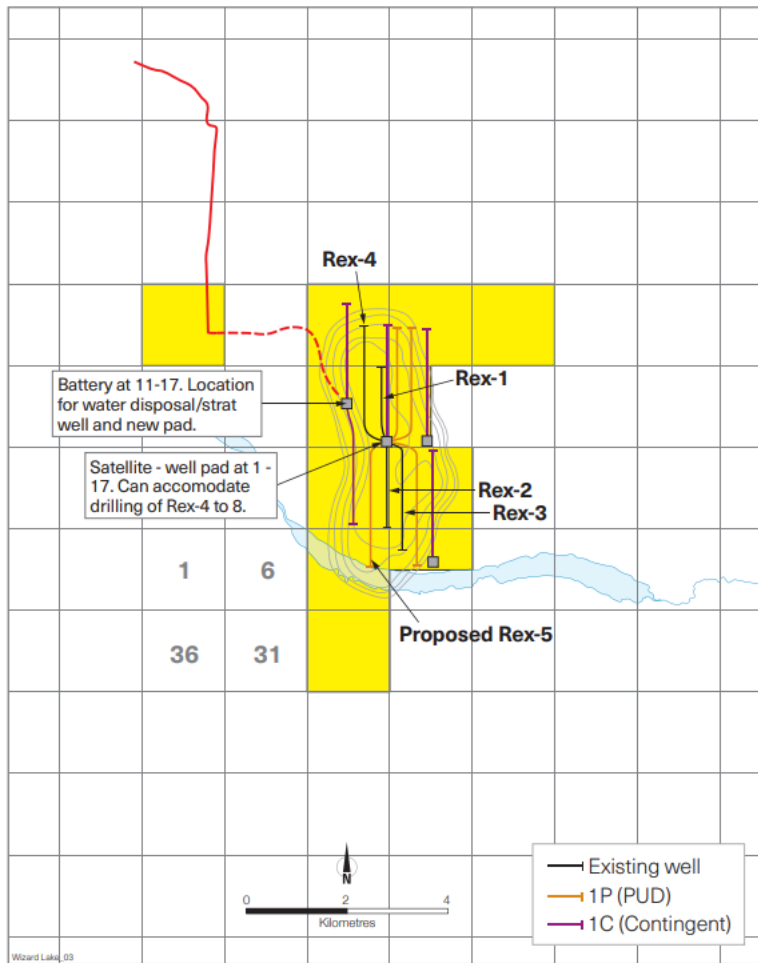
Figure 1 – Wizard Lake Oil Field: Location; Field reservoir map; Existing and planned wellbores
