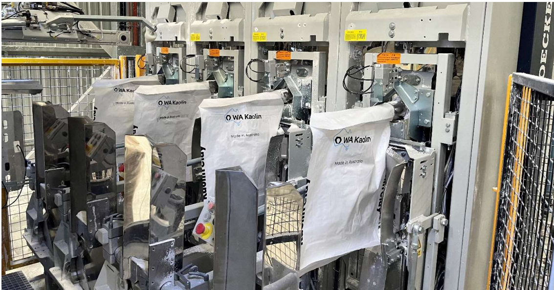
Figure 2 - 20kg bagging station at Wickepin Kaolin Operation
