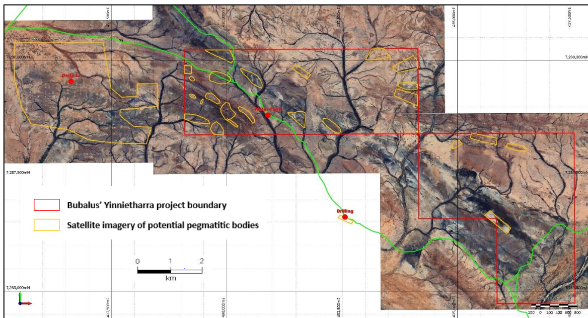
Figure 2. Interpretation of satellite imagery identifies potential pegmatite targets, proximal to Delta Lithium's Malinda Prospect.
