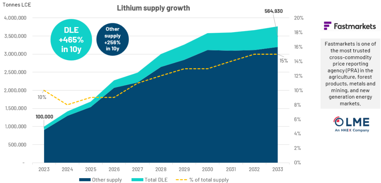
Figure 7 Commercialisation of DLE technology now and into the future.
