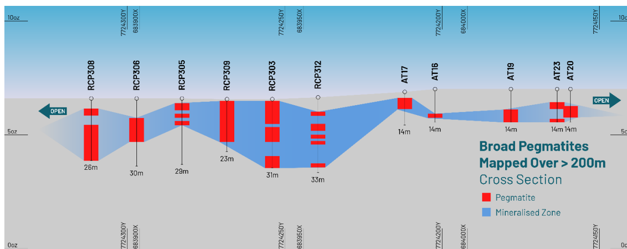
Figure 3: Cross section of historical drilling with pegmatite intersections and interpreted mineralisation zone
