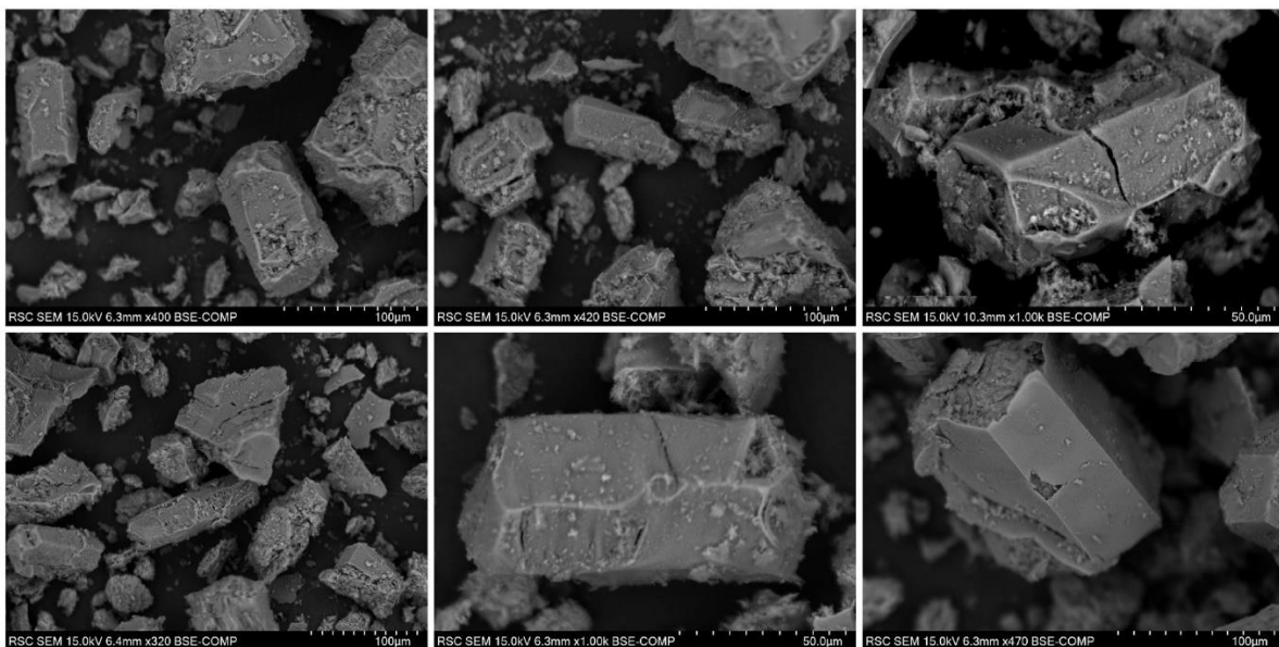
Figure 15. Backscatter scanning electron micrographs of final calcined alumina (sample HY11558) showing corundum crystals and nanoparticles of gamma alumina.
