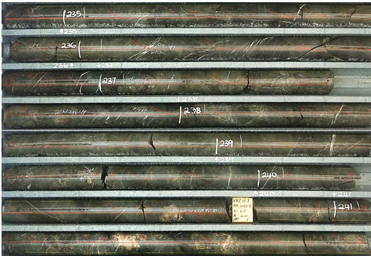
KAI103 (235m – 242m) – Monzonitic intrusive-hydrothermal breccia with calcite-actinolite-chalcopyrite. Photographed interval graded 7m at 1.50g/t AuEq* (0.74% Cu, 0.49g/t Au) from 235m.
