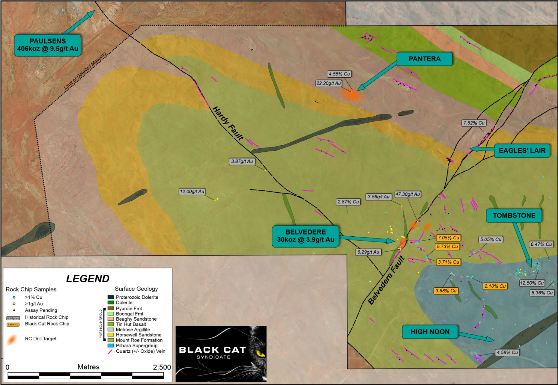
Figure 4: Simplified bedrock geologic map of the Belvedere district showing recent detailed mapping results, the location of historical and recent surface rock samples and the location of pending surface samples. Drill targets for the current RC drill program are also highlighted.
