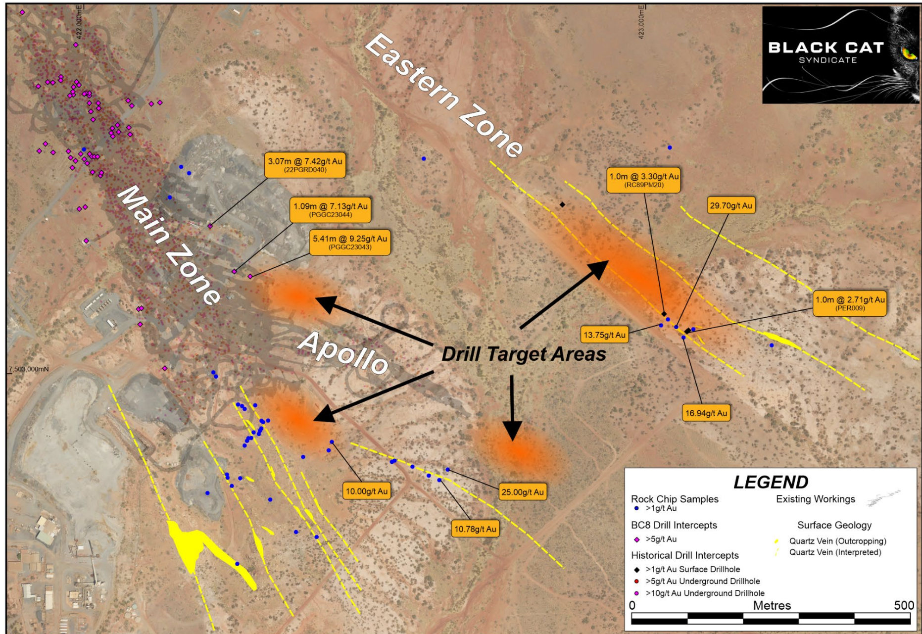
Figure 3: Map showing drill targets at the Eastern Zone and Apollo. Also shown are historical and recent drill intercepts, historical surface samples, the projection of the current mine workings and surface quartz veins.
