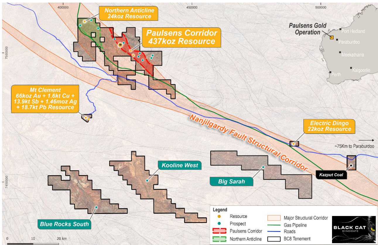
Figure 2: Regional map of the Paulsens Gold Operation showing the location of Resources and large-scale fault architecture.
