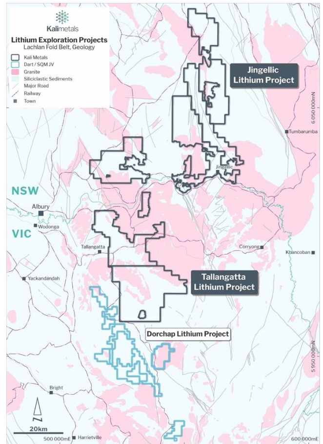
Figure 4: Jingellic Project and Tallangatta Project
