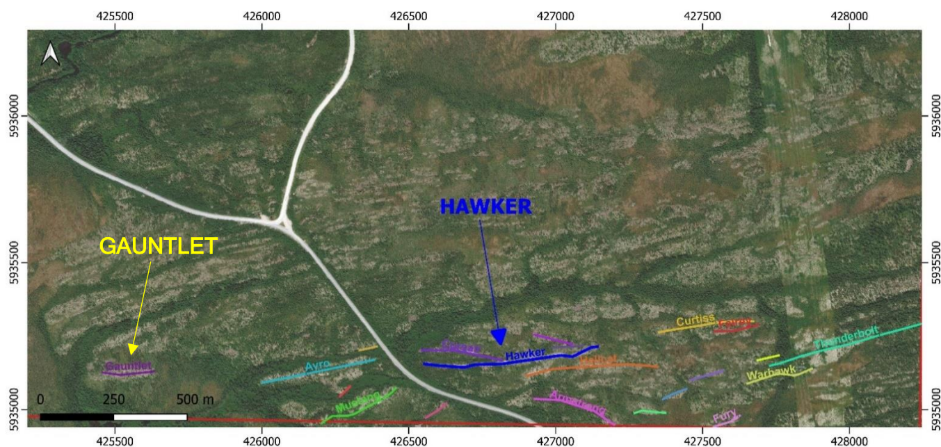
Figure 6 – Pegmatite field at the Aero Property.
