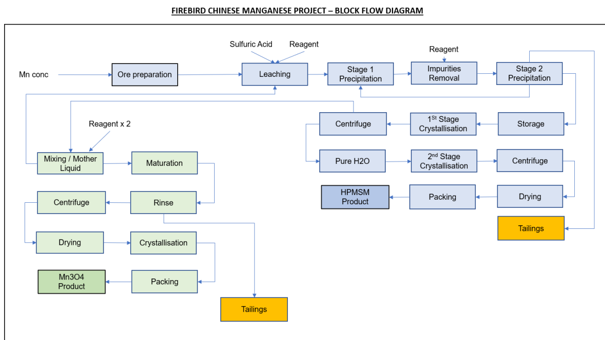
Figure 2: Block flow Diagram
