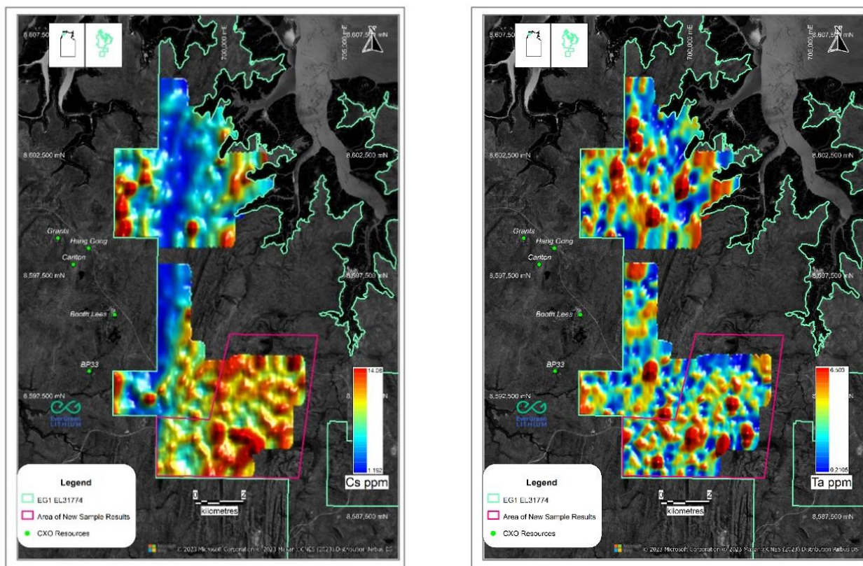
Figure 2 Pathfinder elements Cs and Ta with new soil results highlighted in the pink polygon.
