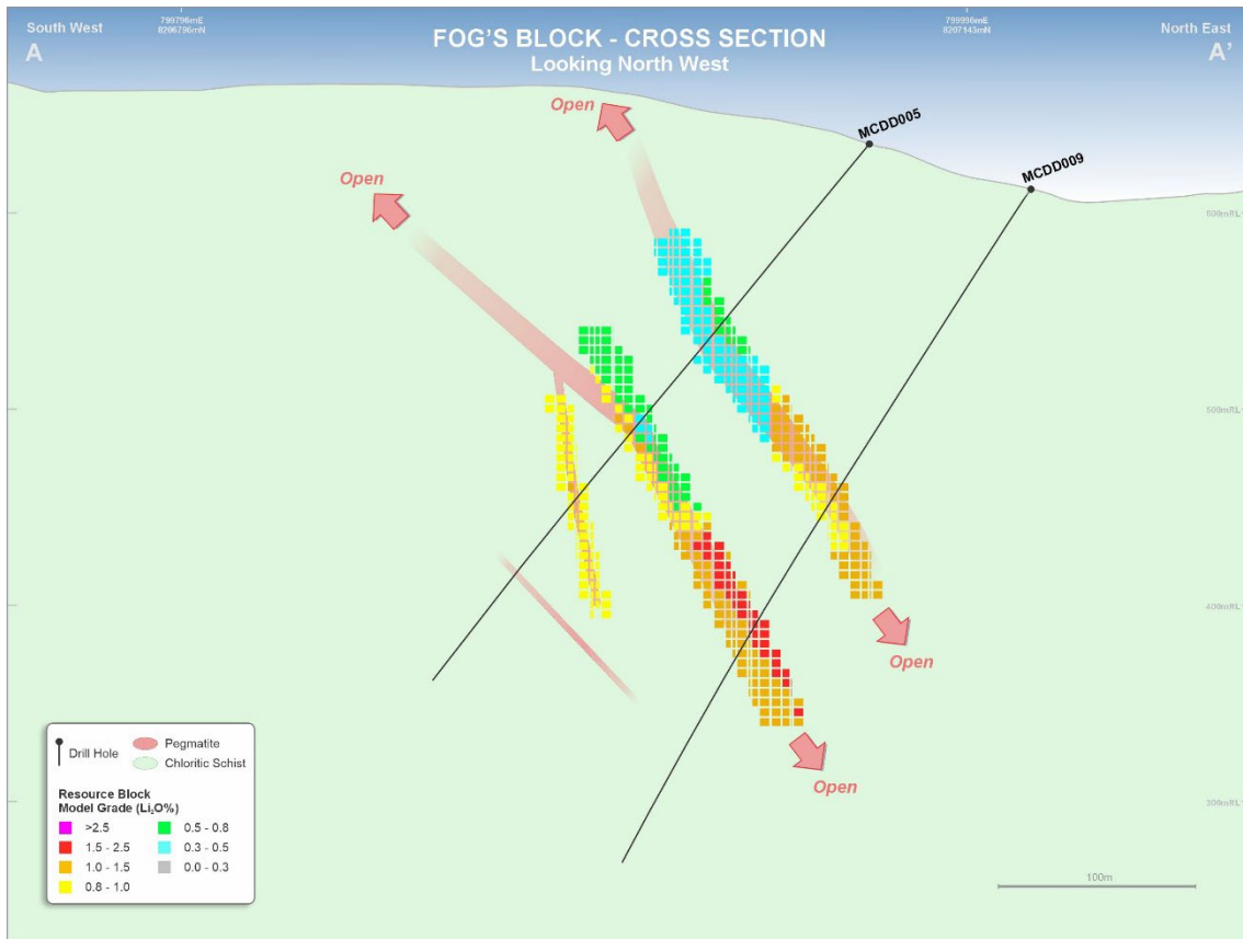
Figure 10: Fog's Block MRE cross section 'A-A'.
