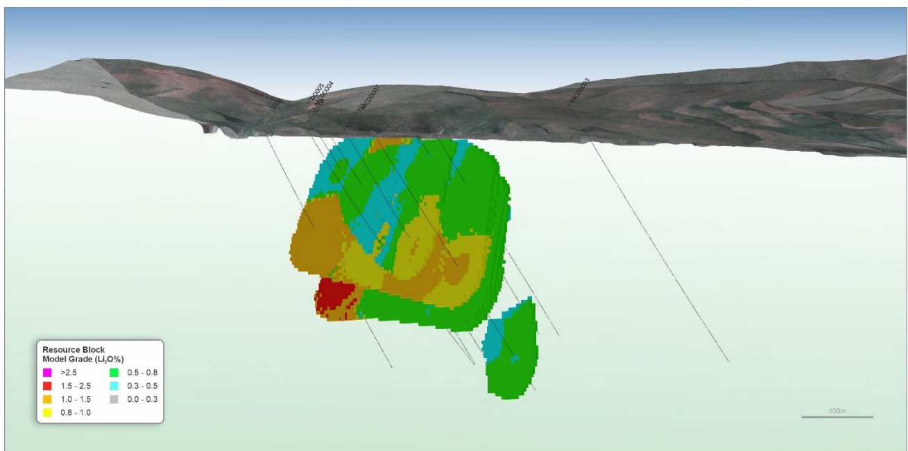
Figure 9: Oblique 3D view of the Fog's Block MRE Model.
