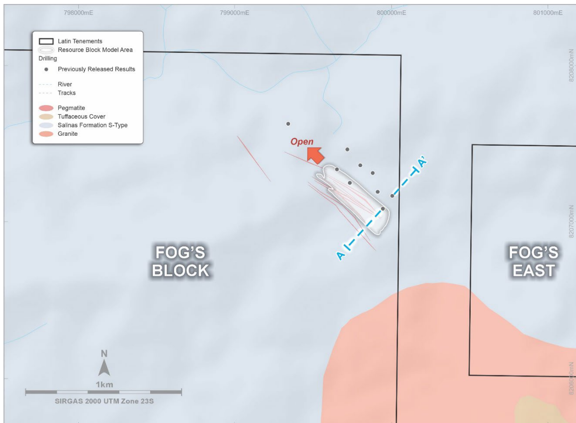
Figure 11: Fog's Block plan view showing the MRE footprint and collars.
