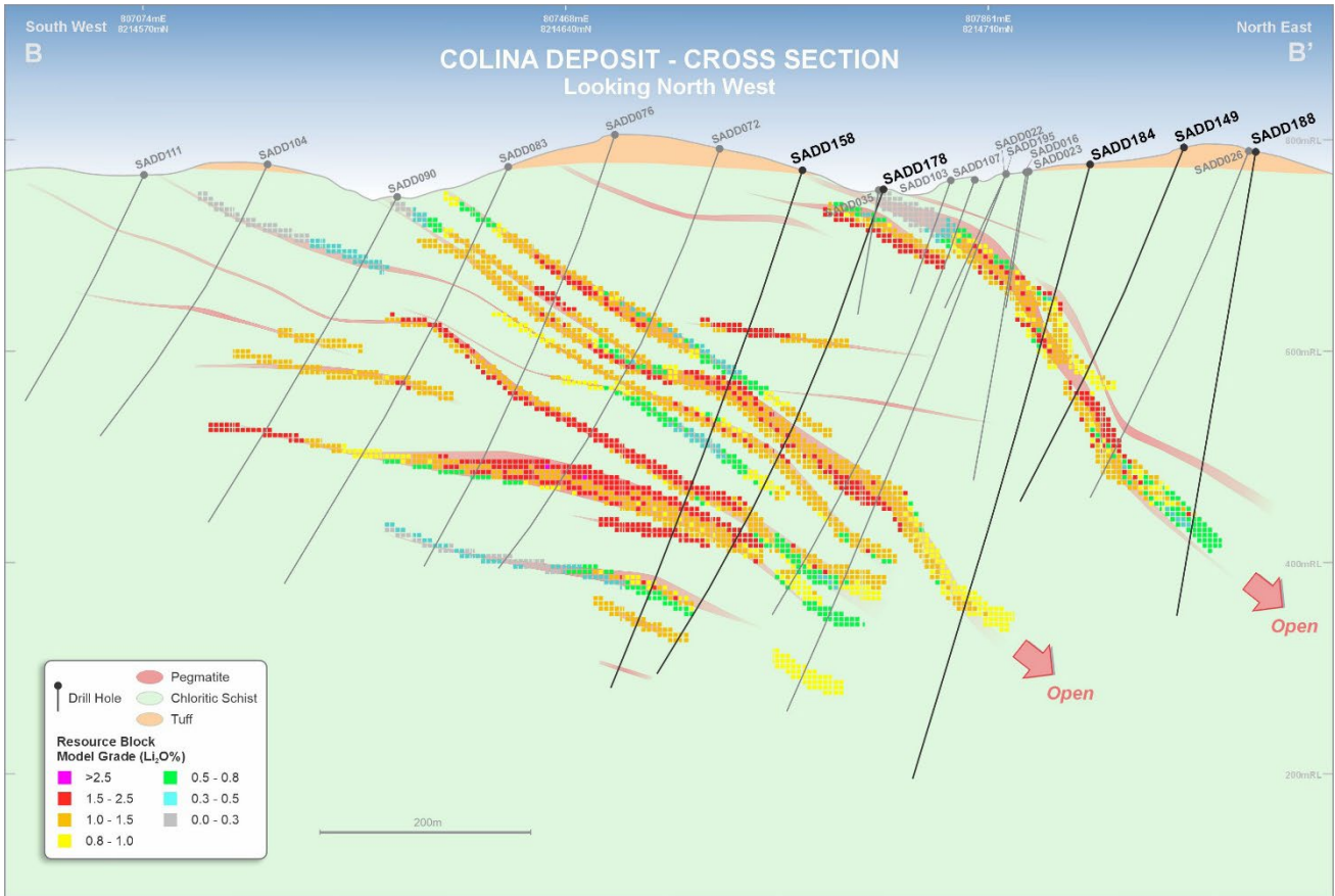
Figure 6: Colina MRE Block Model cross section 'B-B'.
