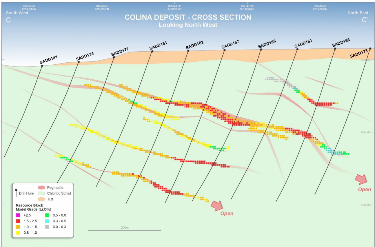
Figure 7: Colina MRE Block Model cross section 'C-C'.
