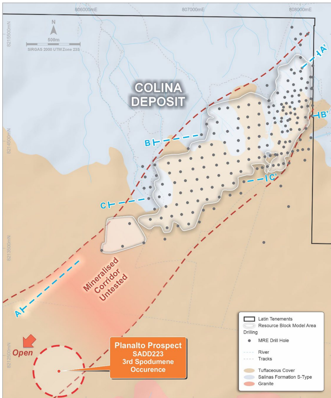
Figure 4: Plan view of the Colina Deposit with MRE area, drill collars and section locations.
