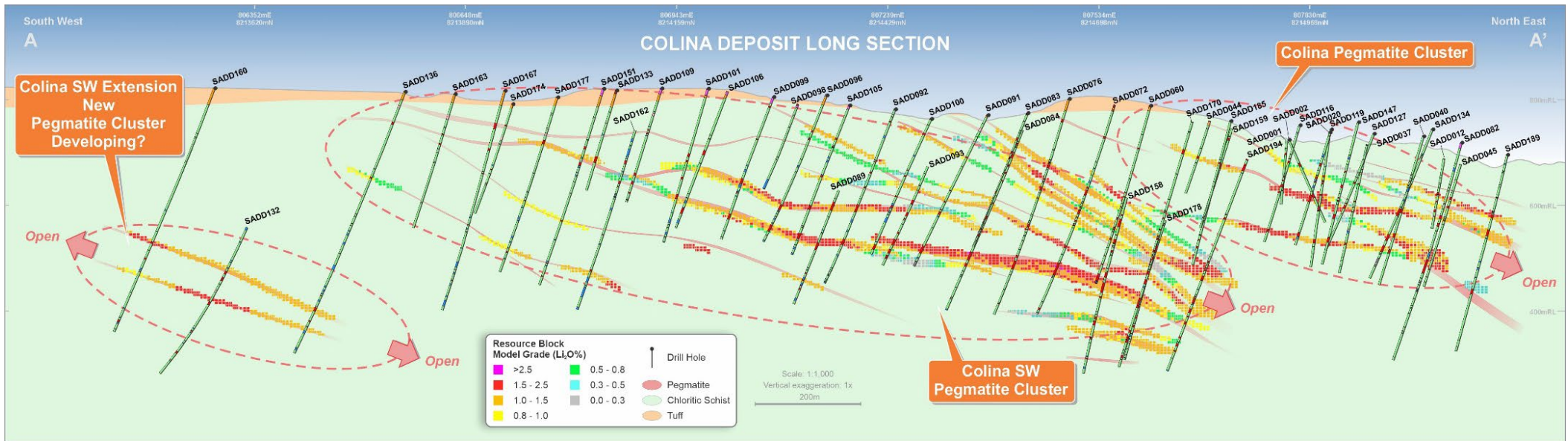
Figure 5: Long Sectional view ('A-A') through the Colina Deposit, showing the updated Colina MRE block model.
