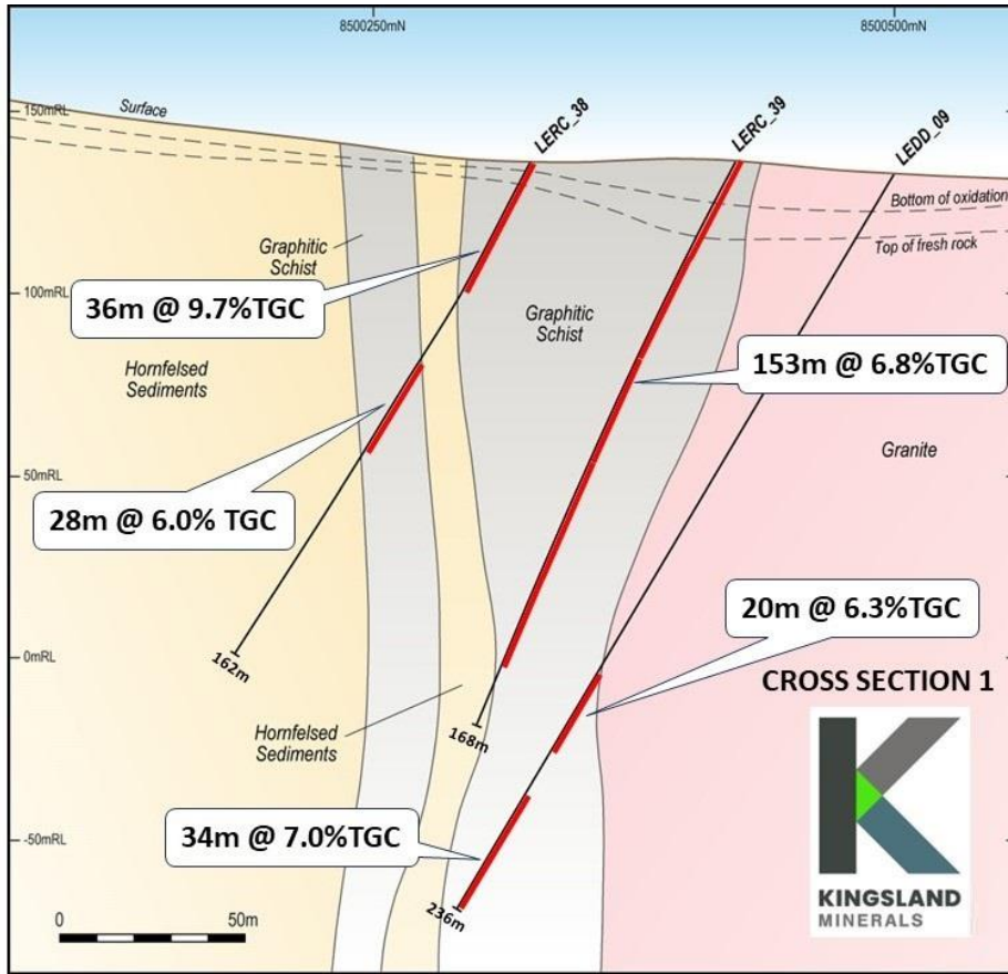
Figure 2: Cross-Section 1 looking north-west
