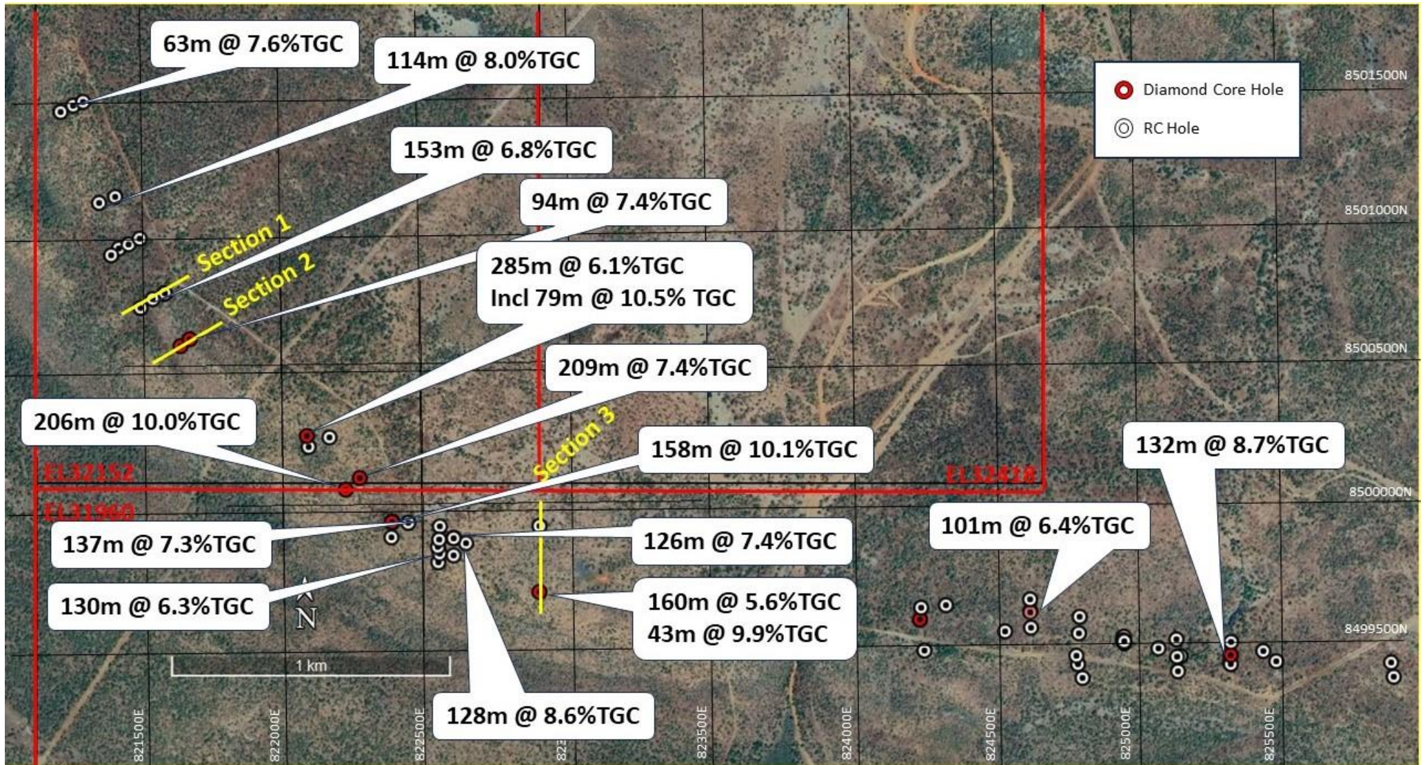
Figure 1: Plan showing location of significant drillhole results and cross sections (MGA Z52)
