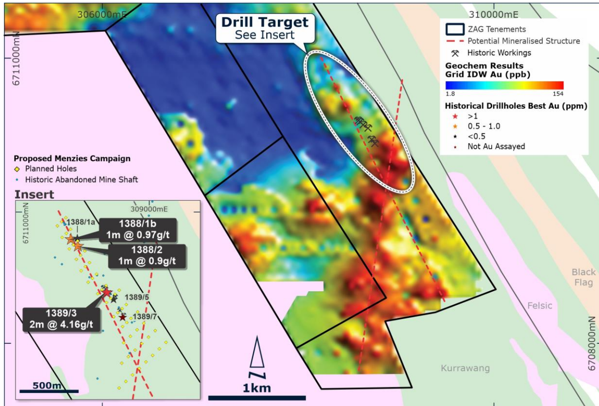
Figure 10 – Menzies soils – contoured gold assays and planned drilling
