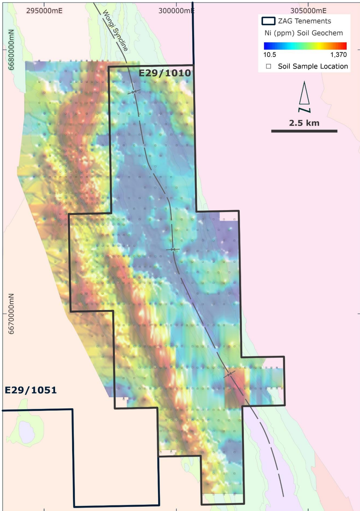
Figure 12 – Goongarrie soils 2022/23 programs - Nickel results
