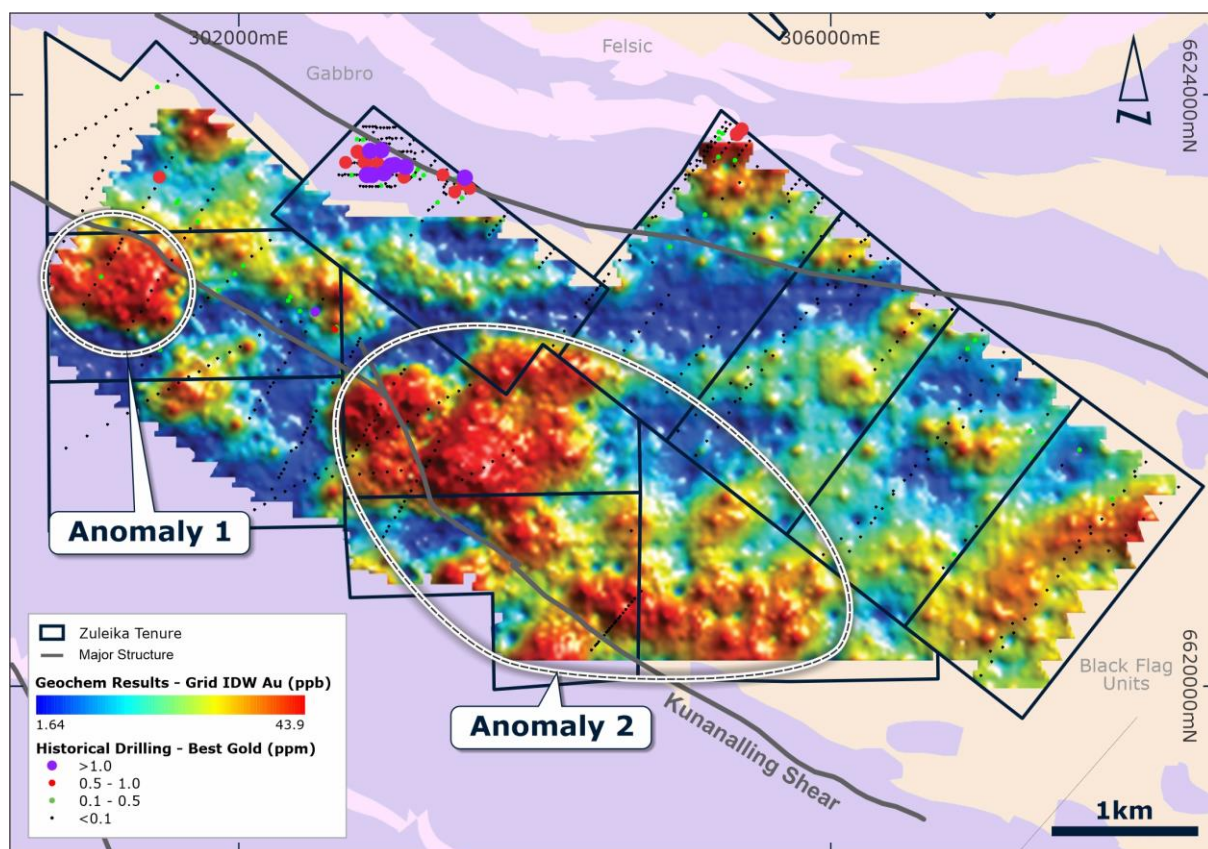
Figure 7 – Breakaway Dam contoured gold geochemistry results
