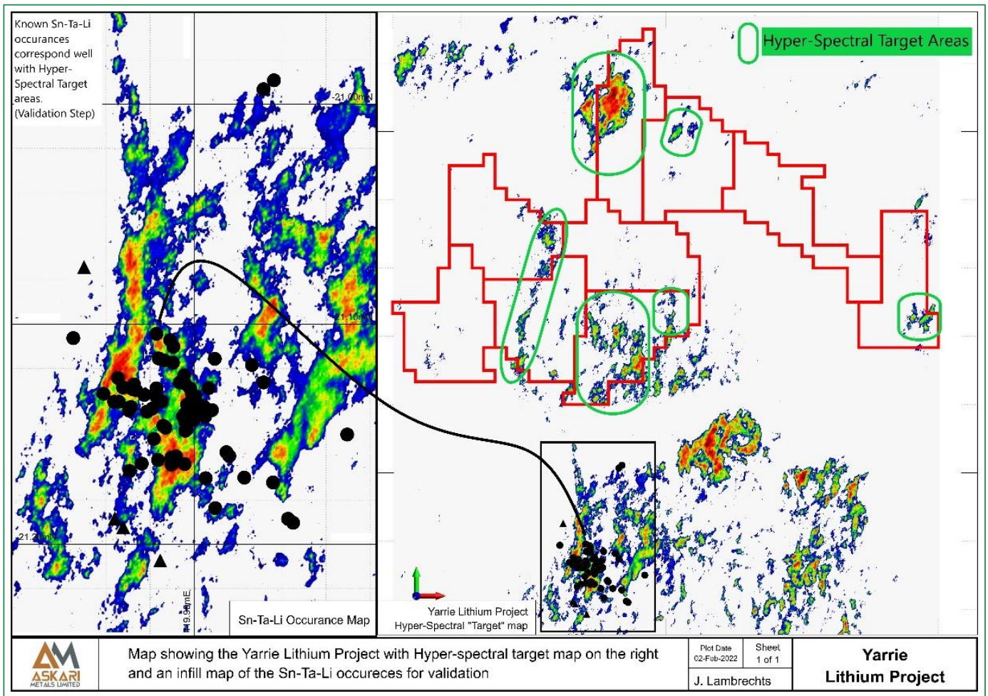
Figure 4: Map depicting targets generated by the hyperspectral analysis of the Yarrarie Lithium Project
