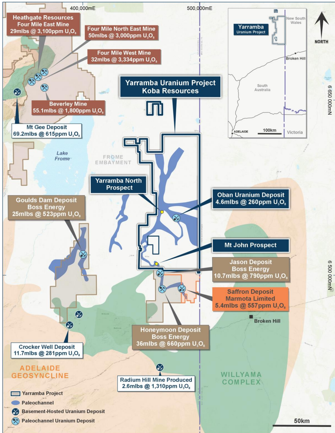
Figure 1. Location of the Yarramba Uranium Project within a world-class uranium district in South Australia. 1234567
