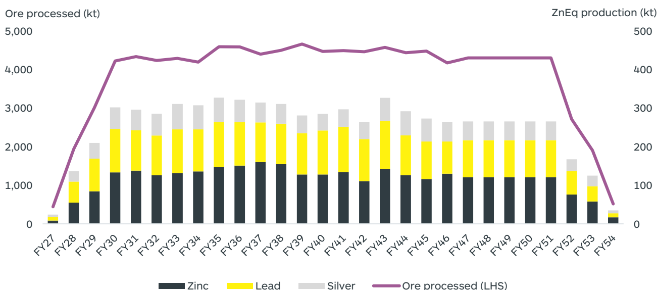
Figure 3: Ore processed and payable ZnEq production
