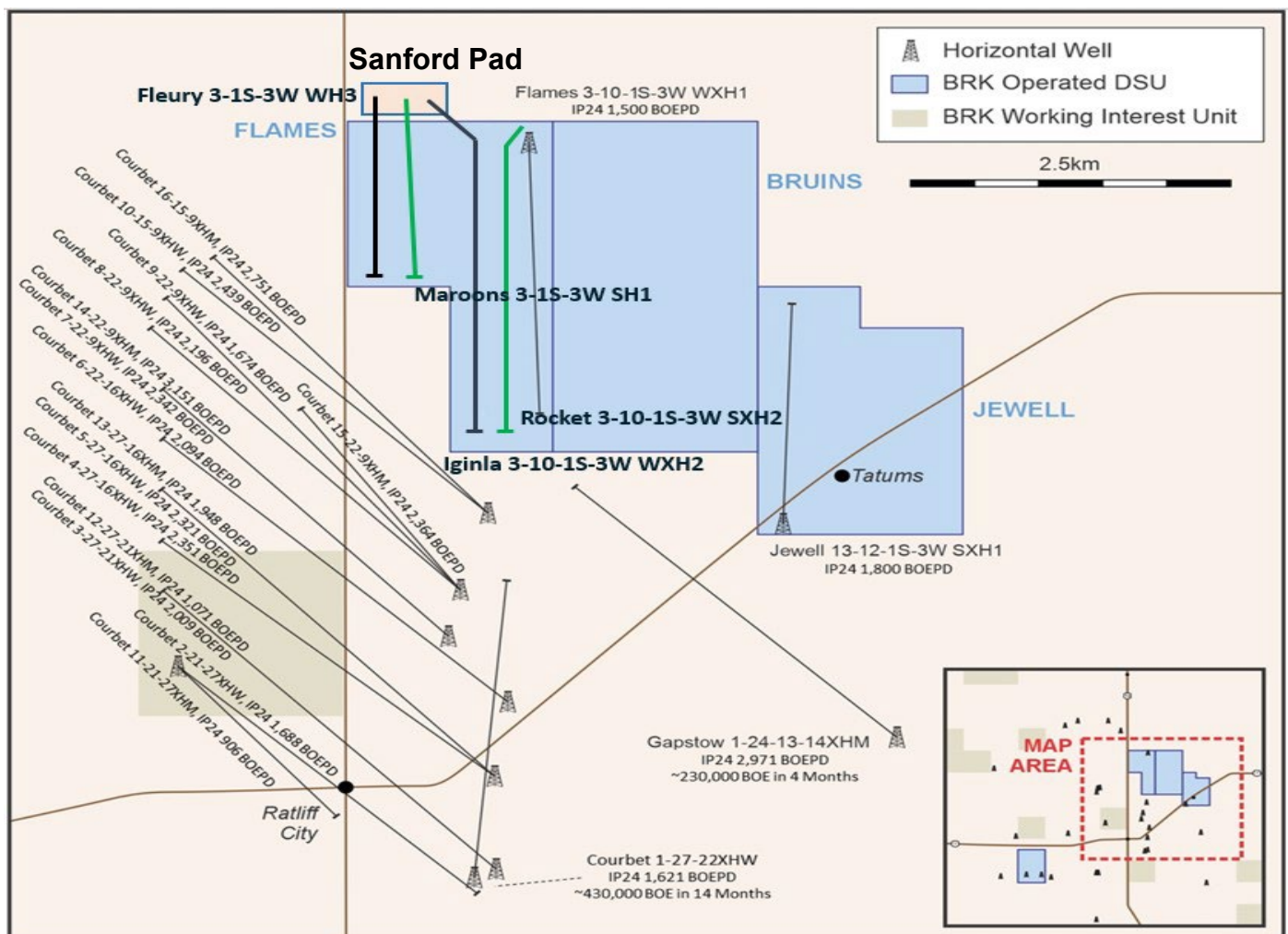
Figure 2: Location of the Sanford Pad and the four FMDP wells: Fleury, Maroons, and Iginla Wells (to be drilled from the Sanford Pad), and the Rocket Well (to be drilled from the existing Flames Well pad). Also shown are Continental Resources Courbet Wells full field development showing the strong performance of both the Woodford wells (well names ending with XHW) and Sycamore wells (well names ending in XHM).
