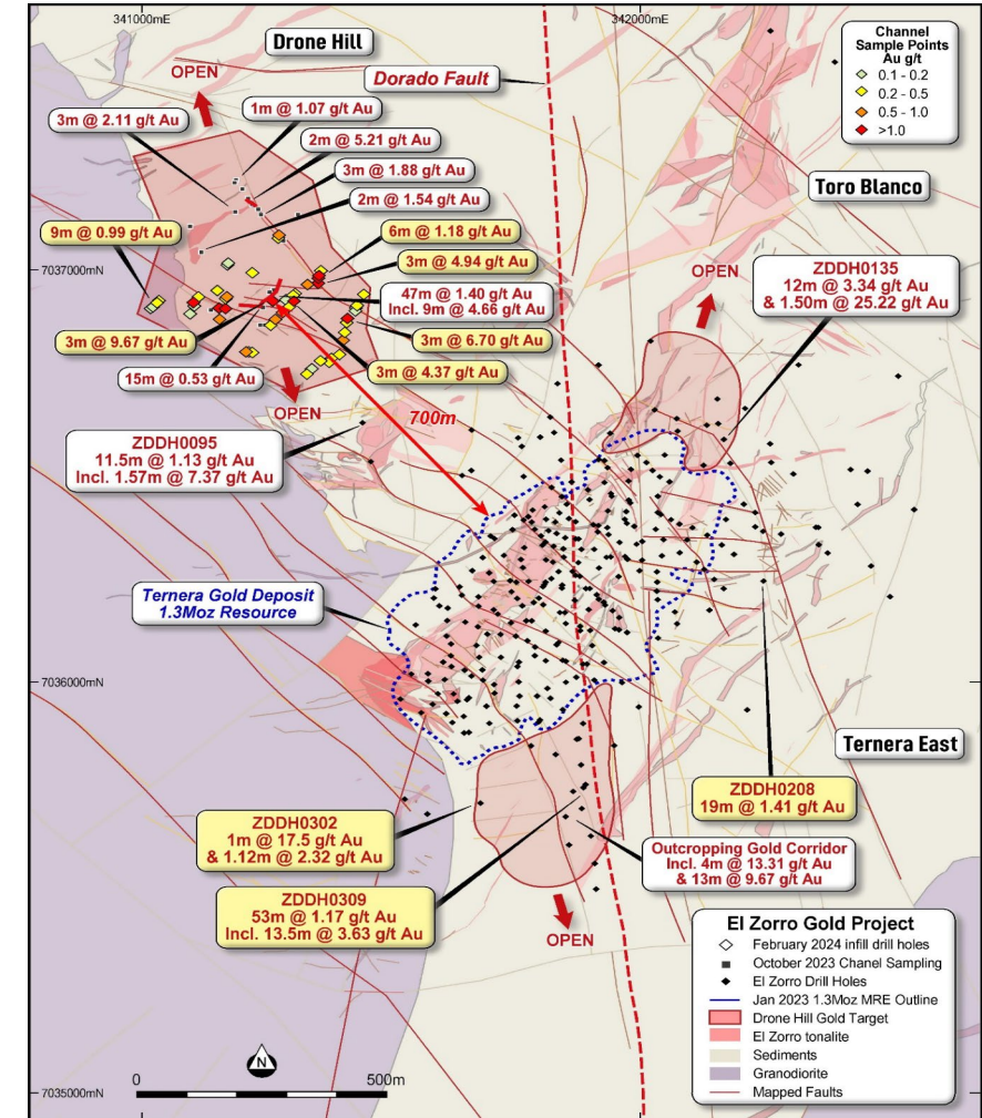
Ternera Gold Deposit – near deposit targets highlighting significant drill intercepts and sampling results from high priority areas
