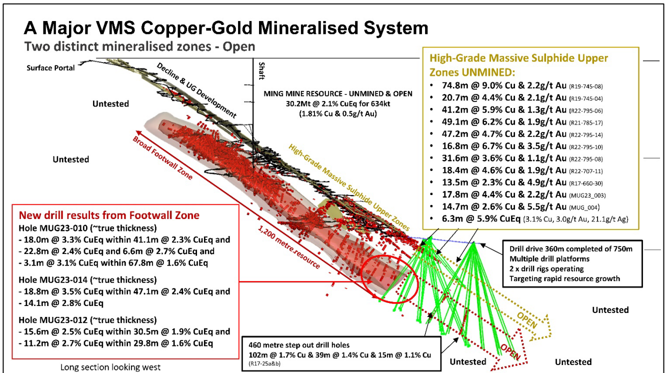
Figure 2: Long Section through the Green Bay Ming Mine showing the location of the FireFly Metals Footwall Zone drilling and planned drilling for 2024. Refer to ASX releases dated 31/8/23, 11/12/23 and 16/1/24 for details of previous results.
