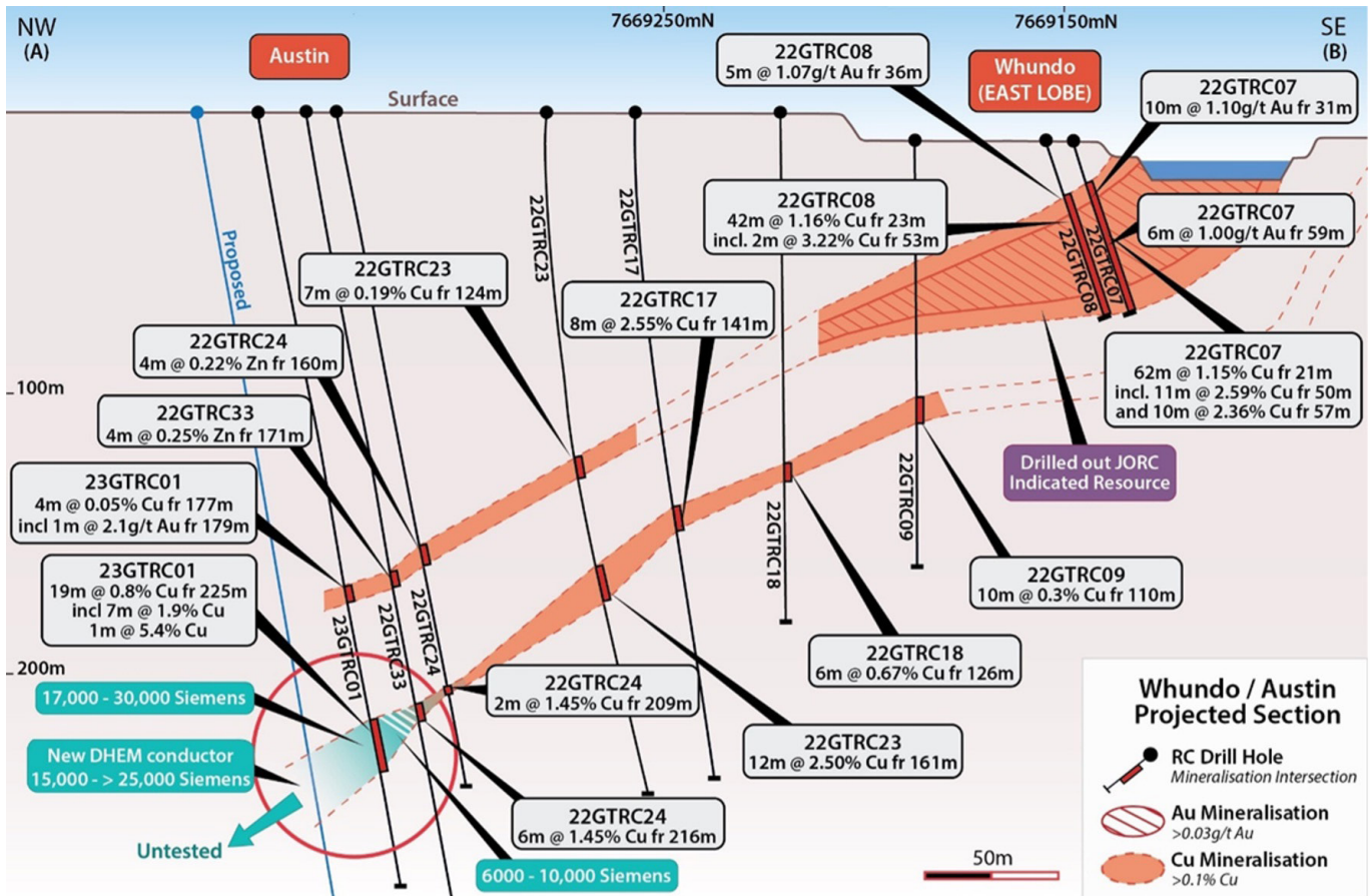
Figure 8. Whundo-Austin Section
