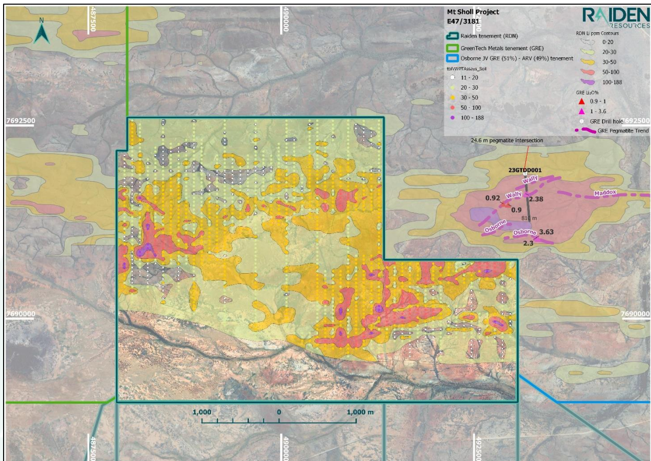
Figure 1: Mt Sholl Project with the results of Raiden’s lithium infill soil sampling program, in relation to GreenTech Metals Ltd.’s Osbourne JV results 1,2
