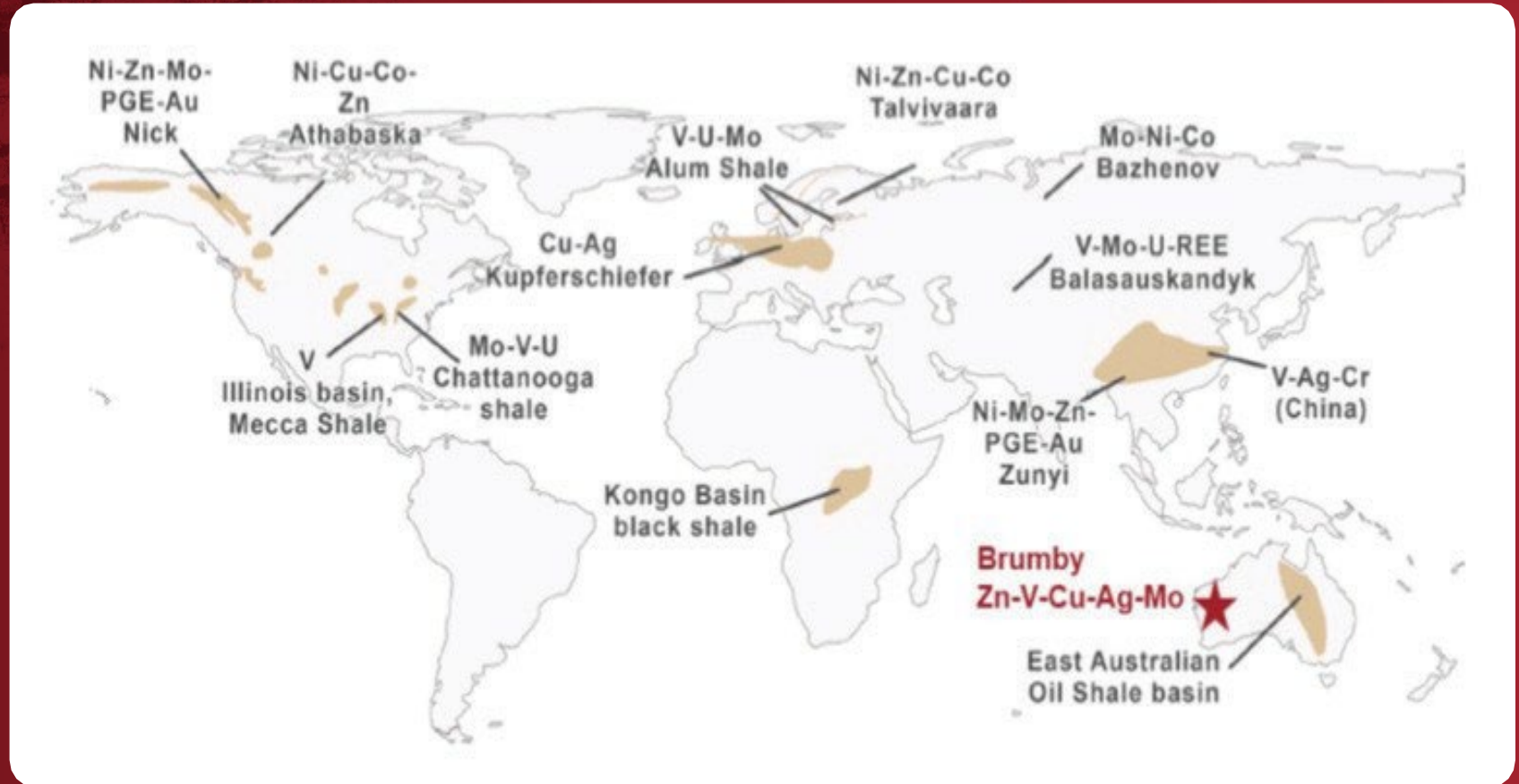
Major black shale districts (brown areas) and a selection of significant deposits across the world. Compiled after (Convey and PaŠava, 2004) and (Large, 2012).
