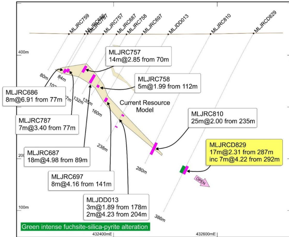
Figure 5. Cross section for LNJ4 northern area showing high-grade dipping gold zone containing resource model outline and MLRCD829 being a down dip extension of over 75m with intense fuchsite alteration.
