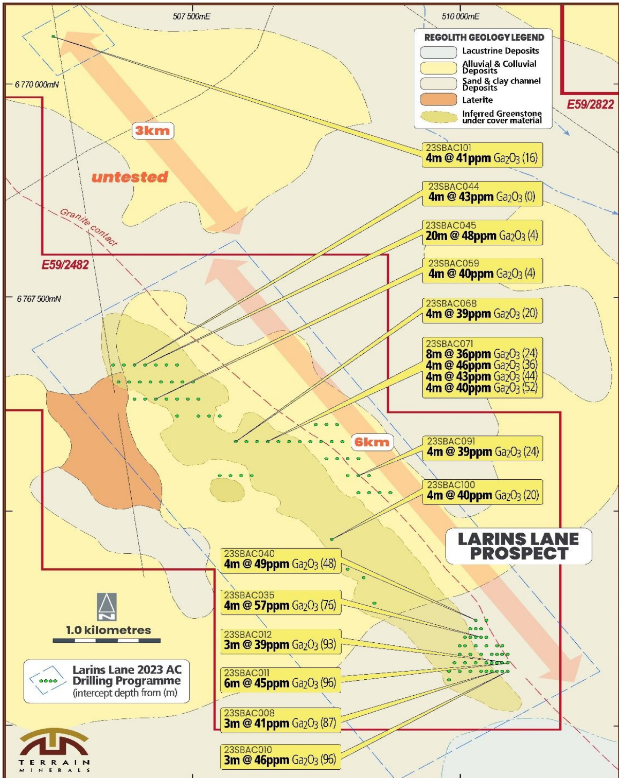
Diagram 7: Drill hole location of Terrain’s 2023 air core drill program at the Larins Lane Project with selected gallium oxide grades highlighted. Warning: Most holes remain open and untested.
