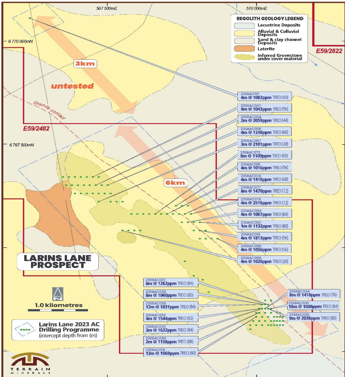
Diagram 6: Drill hole location of Terrain’s 2023 air core drill program at the Larins Lane Project with selected REE grades highlighted. Warning: Most holes remain open and untested.
