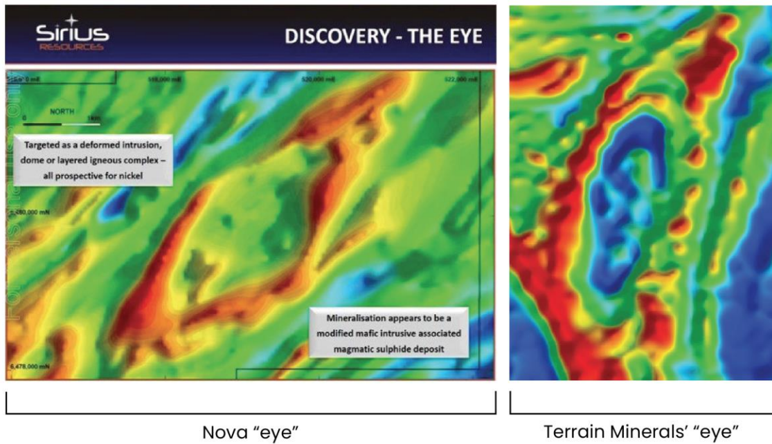
Diagram 3. Host geology of the Nova-Bollinger nickel-copper orebody appears as a very distinctive 'EYE' in the aeromagnetic data (left image). Terrain has identified a possible repetition of the Nova-style eye feature within its recently granted tenement E63/2447 (right image) (Source: Sirius Resources' ASX announcement dated 4 October 2012).
