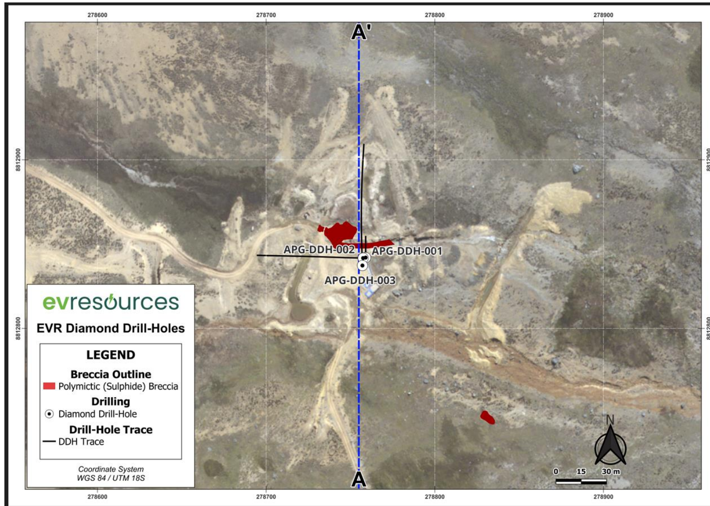
Figure 5: Plan view from Trincheras Este Breccia zone, APG-DDH-001 and APG-DDH-003
