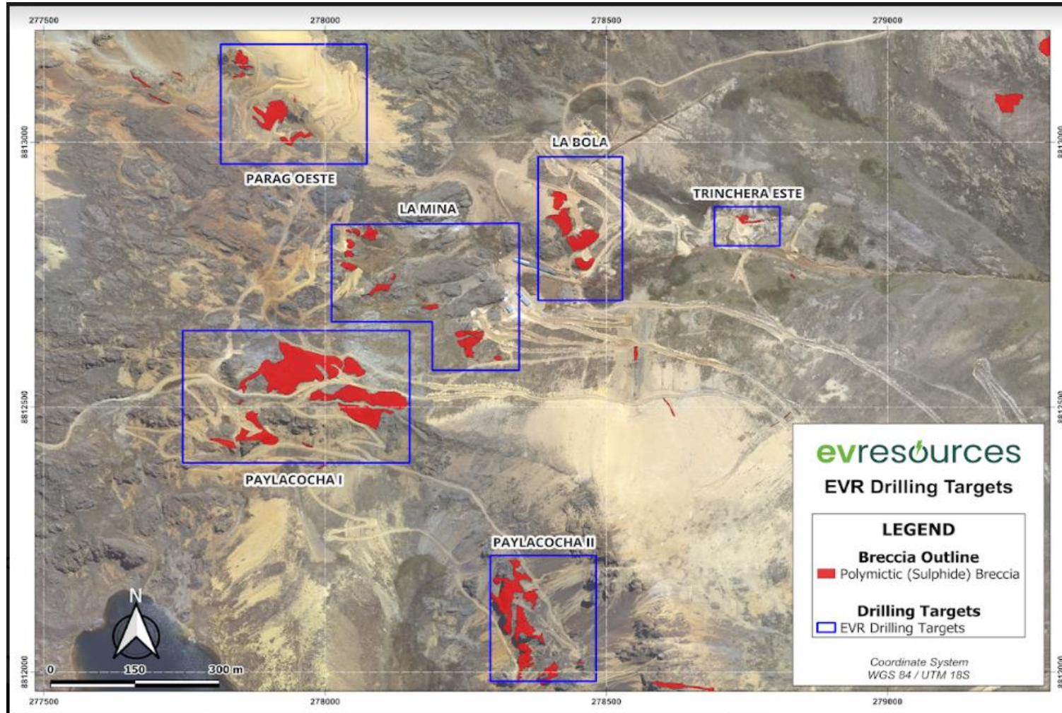
Figure 4: Plan view of the location of breccia bodies
