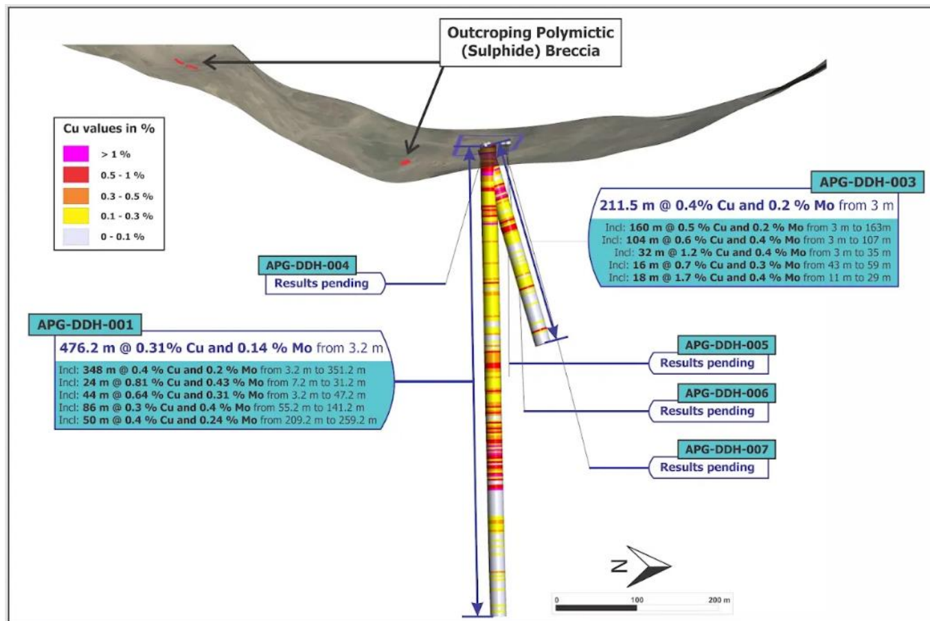
Figure 2. 3D view with Cu intervals, Holes APG-DDH-003 *
