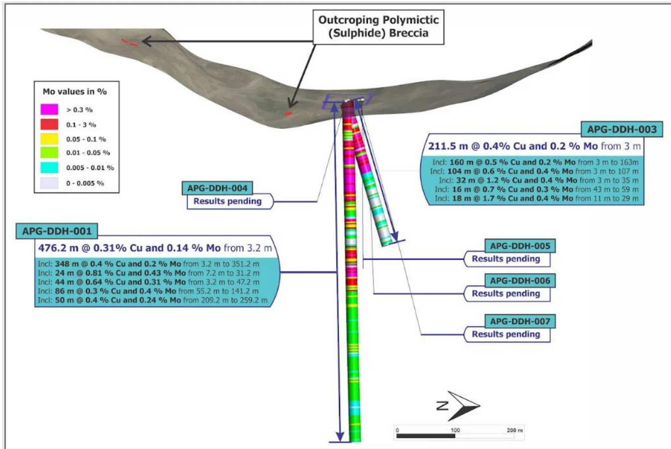
Figure 3. 3D view with Mo intervals, Holes APG-DDH-003 *
