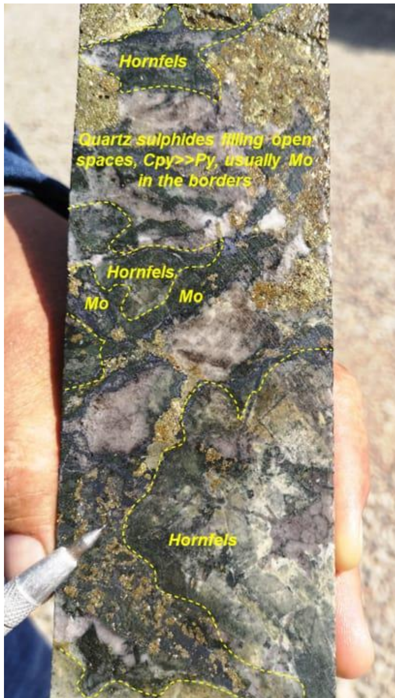
Sample 00471 at 51.80m, with 1.14%Cu and 0.5955%Mo
