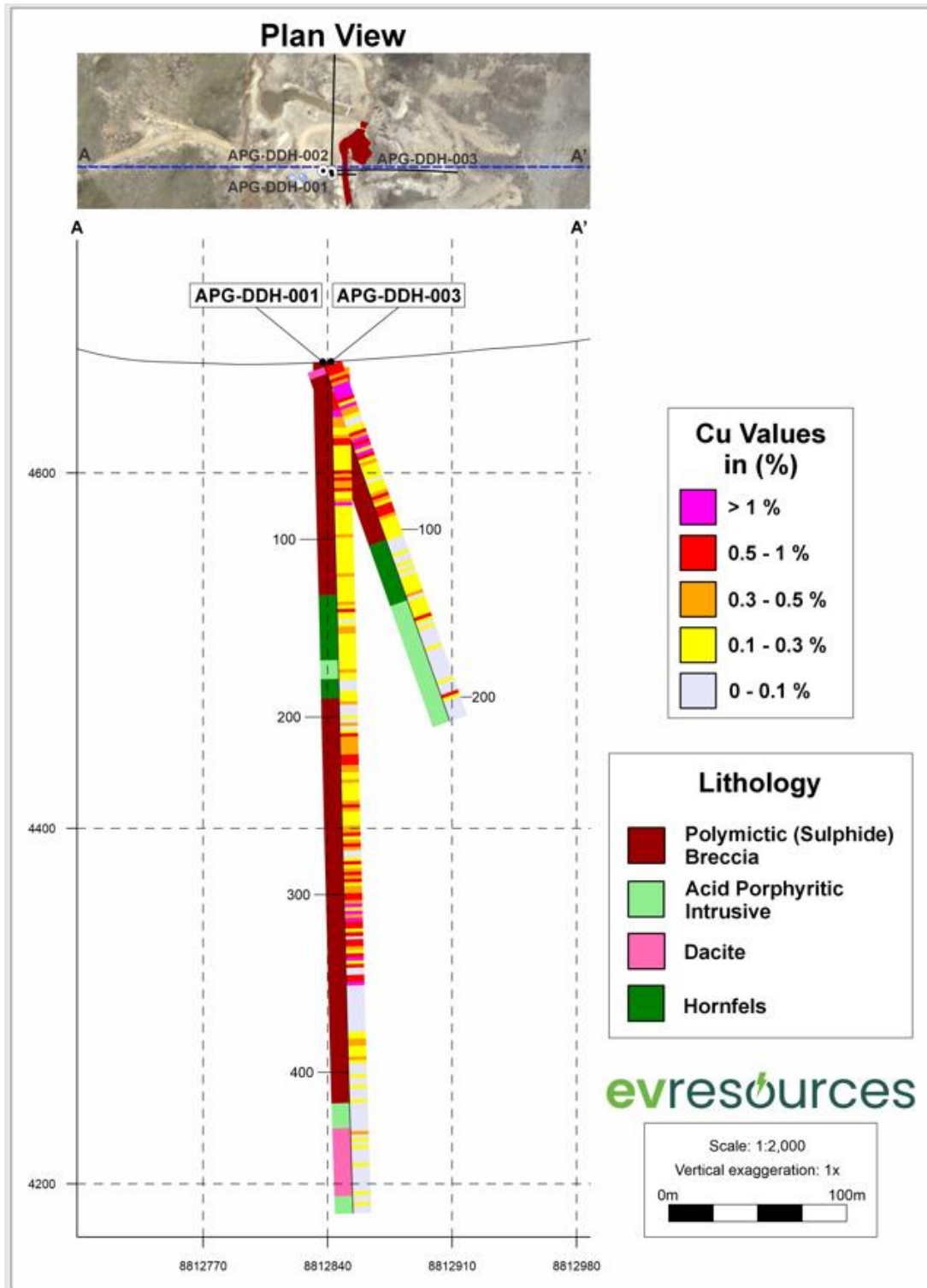
Figure 6: Cross Section along A-A' looking West, Hole APG-DDH-003, downhole copper assay values, 2 m interval.
