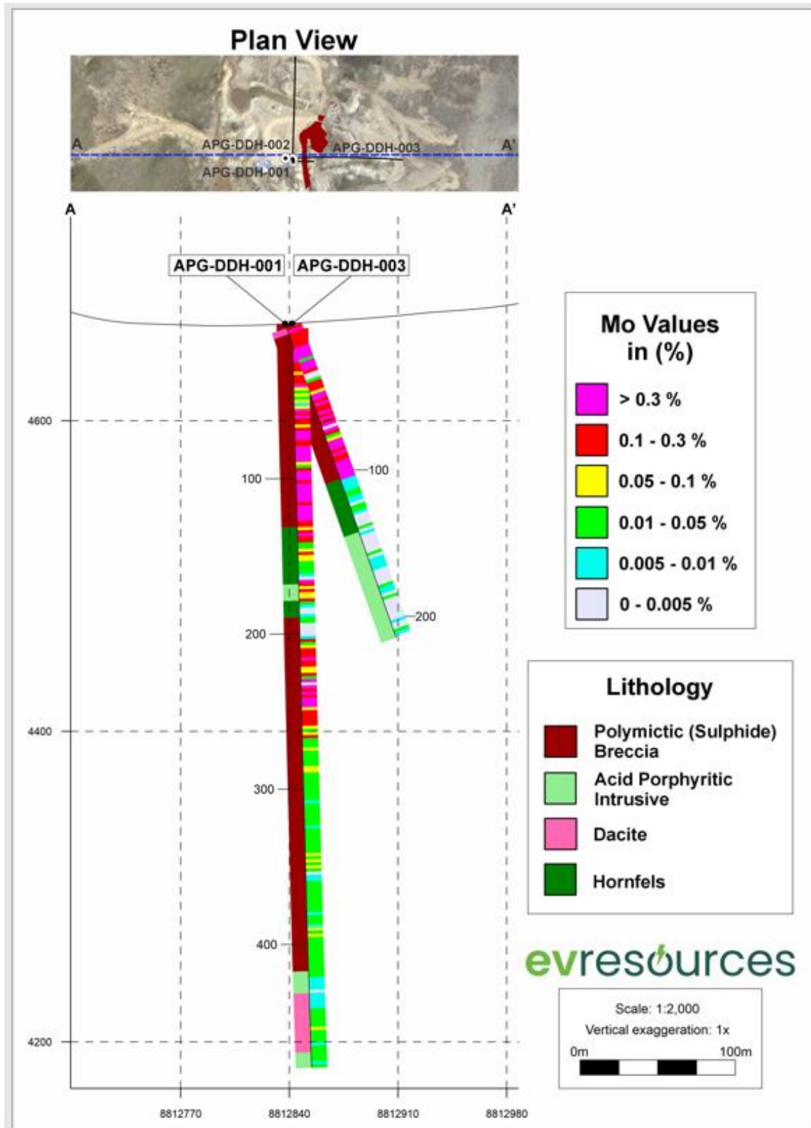
Figure 7 Cross Section along A-A' looking West, Hole APG-DDH-001 and APG-DDH-003 Down hole molybdenum assays values, 2 m interval.
