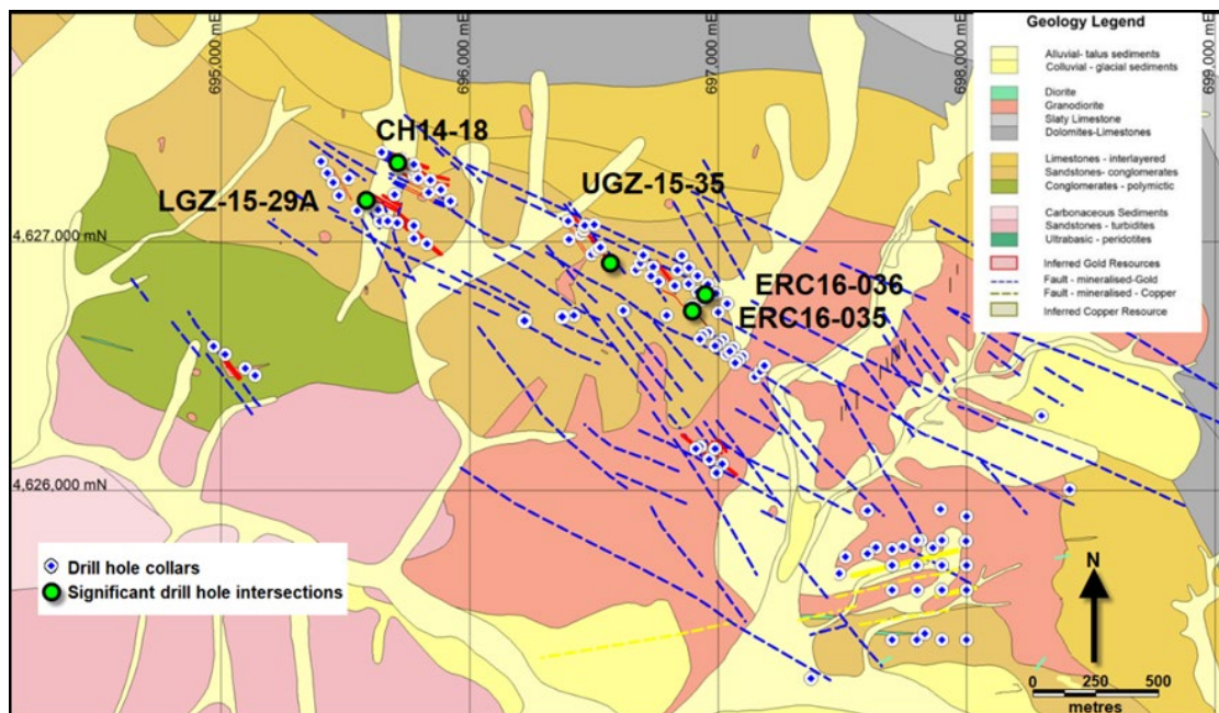
Figure 3: Locations of Significant Drill Intercepts at Chanach Gold Project Mineral Resource
