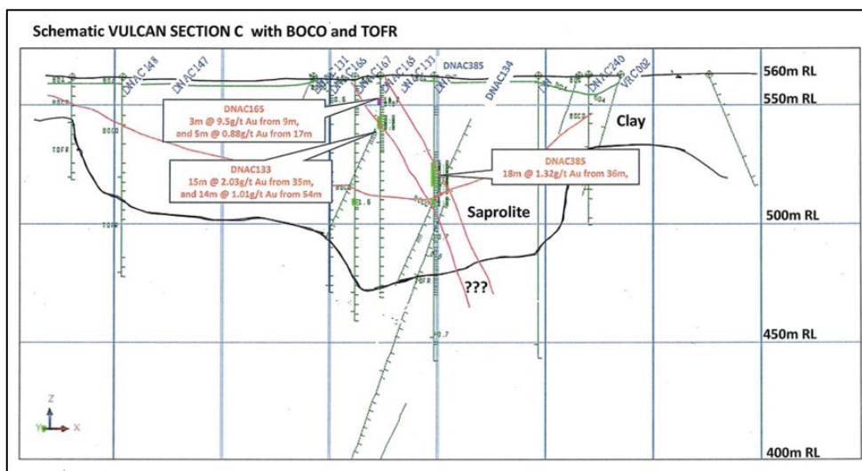
Figure 3. E52/2049 – Example - Cross Section - Vulcan Air Core Drill Intersections
