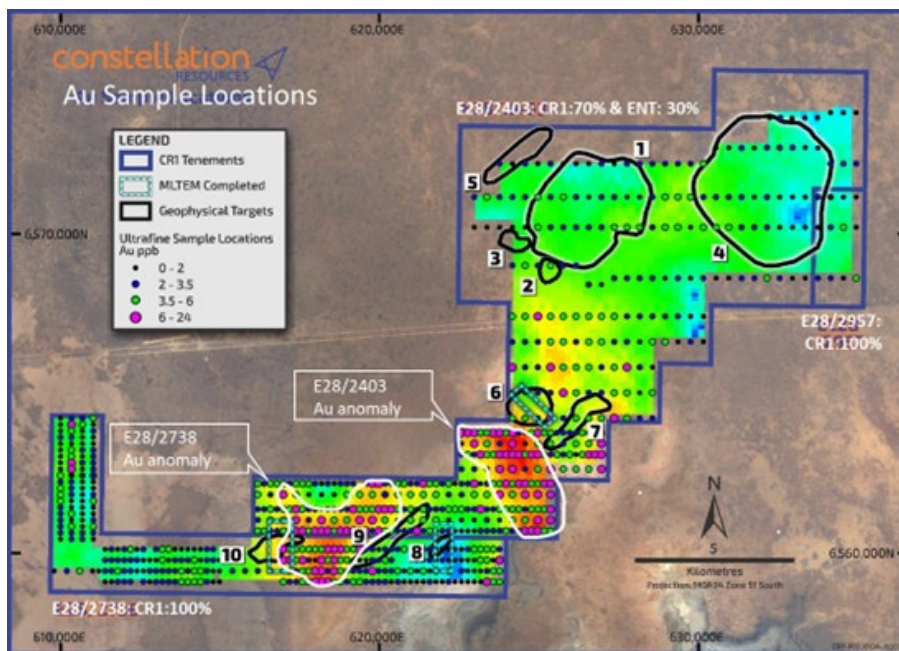
Figure 5. Ultrafine Soil Sampling Results over Transline Tenements with Anomalous Gold (Au) Gridded Base Image and Previously Identified Geophysical Targets
