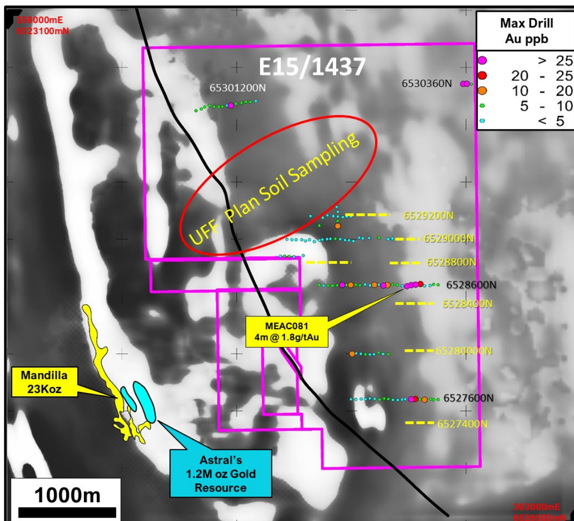
Figure 1. E15/1437 - 1 st VD Magnetic Image with Enterprise’s 2022 Air Core Holes
