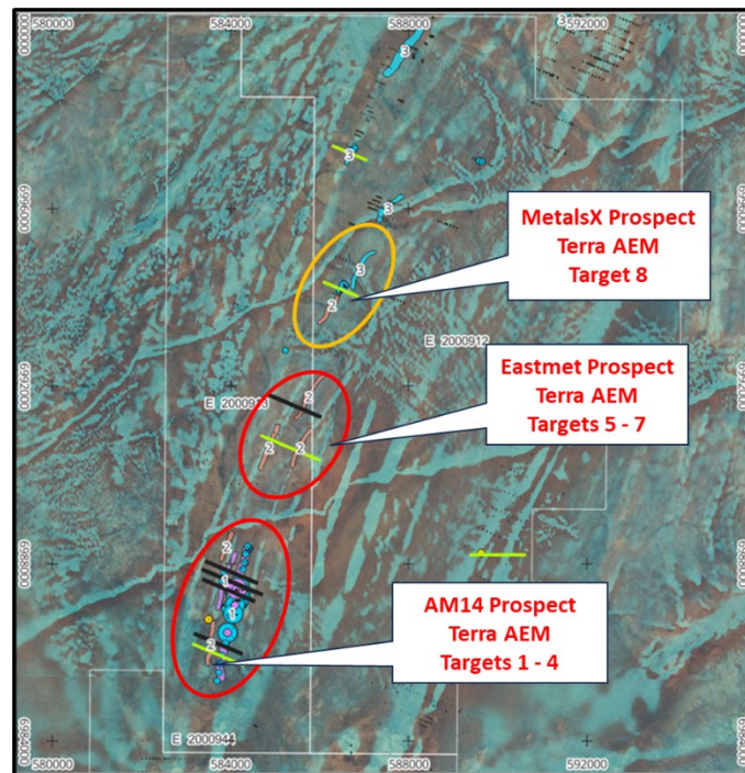
Figure 3. Location of 2022 AEM Targets with Historic Down Hole Geochemistry.
