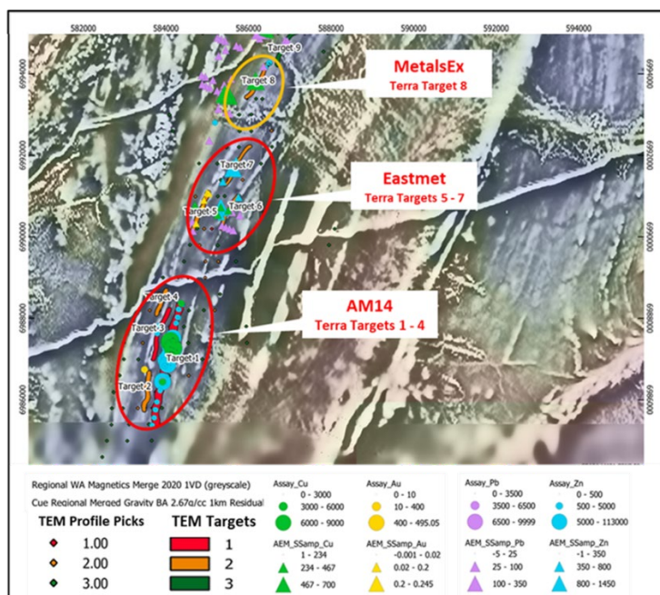
Figure 3. Location of 2022 AEM Targets with Historic Down Hole Geochemistry.
