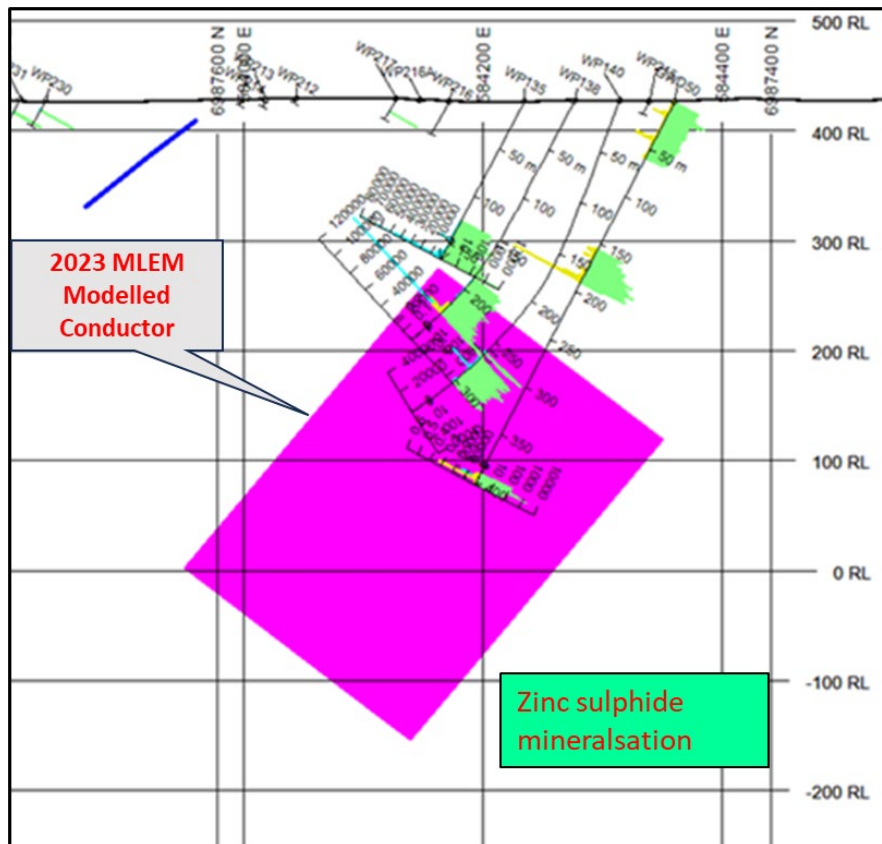
Figure 4. Cross Section of AM14 Prospect with Historic Drillholes and 2023 MLEM Modelled Conductor.
