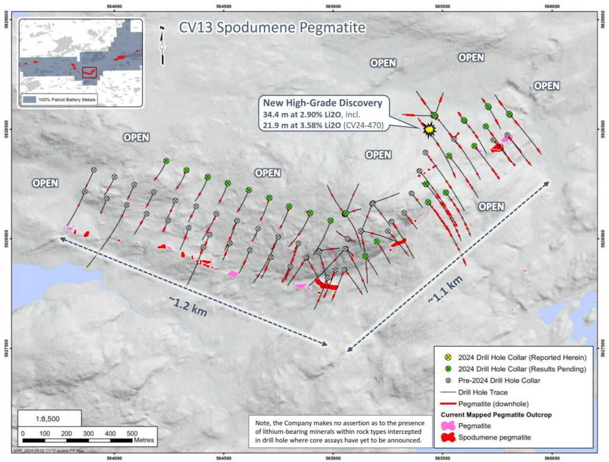
Figure 2: Drill holes completed at the CV13 Spodumene Pegmatite through April 2024.
