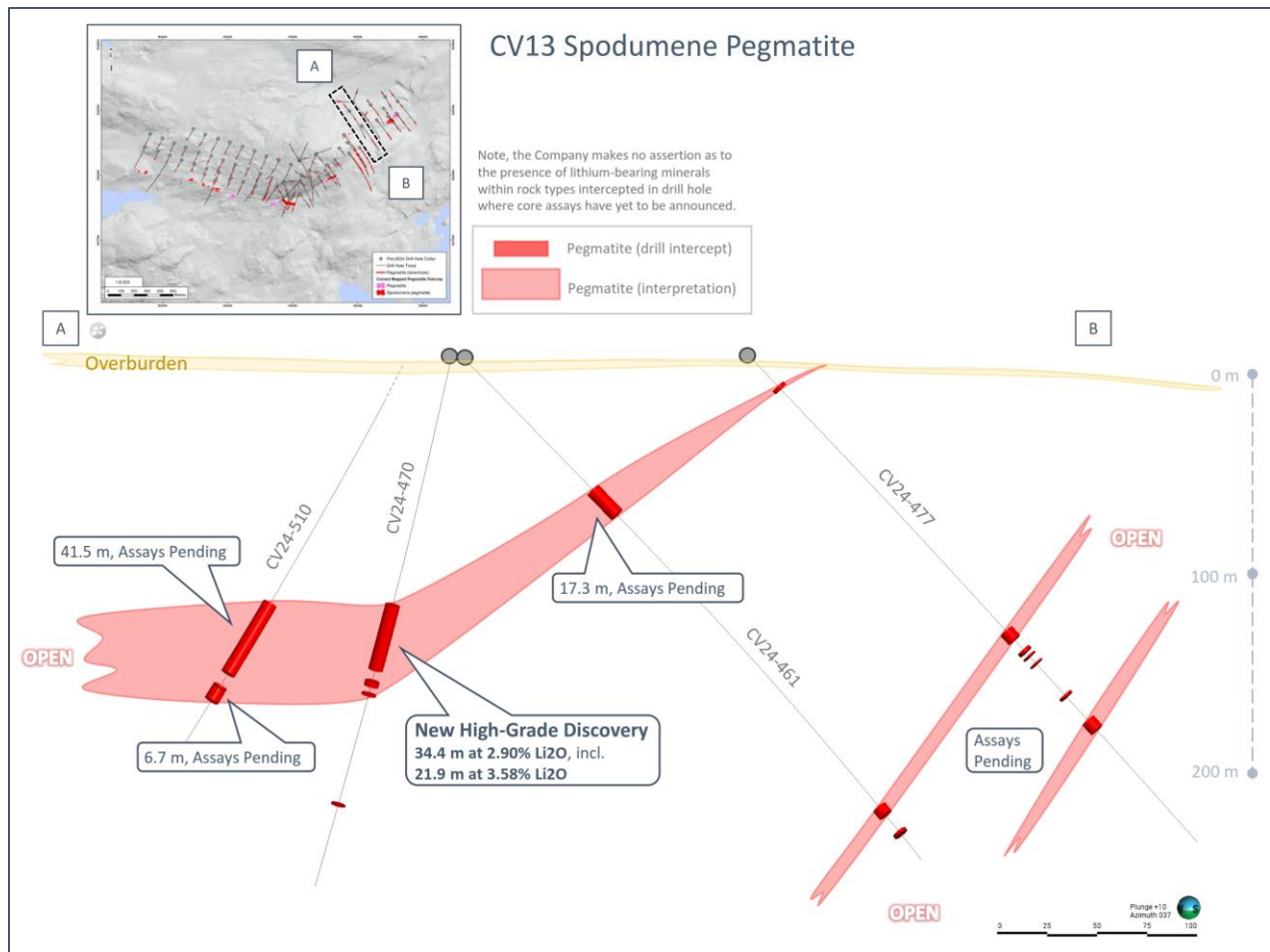
Figure 1: Preliminary cross-section of the CV13 geological model at the end of the April 2024 program. Results announced herein for drill hole CV24-470.
