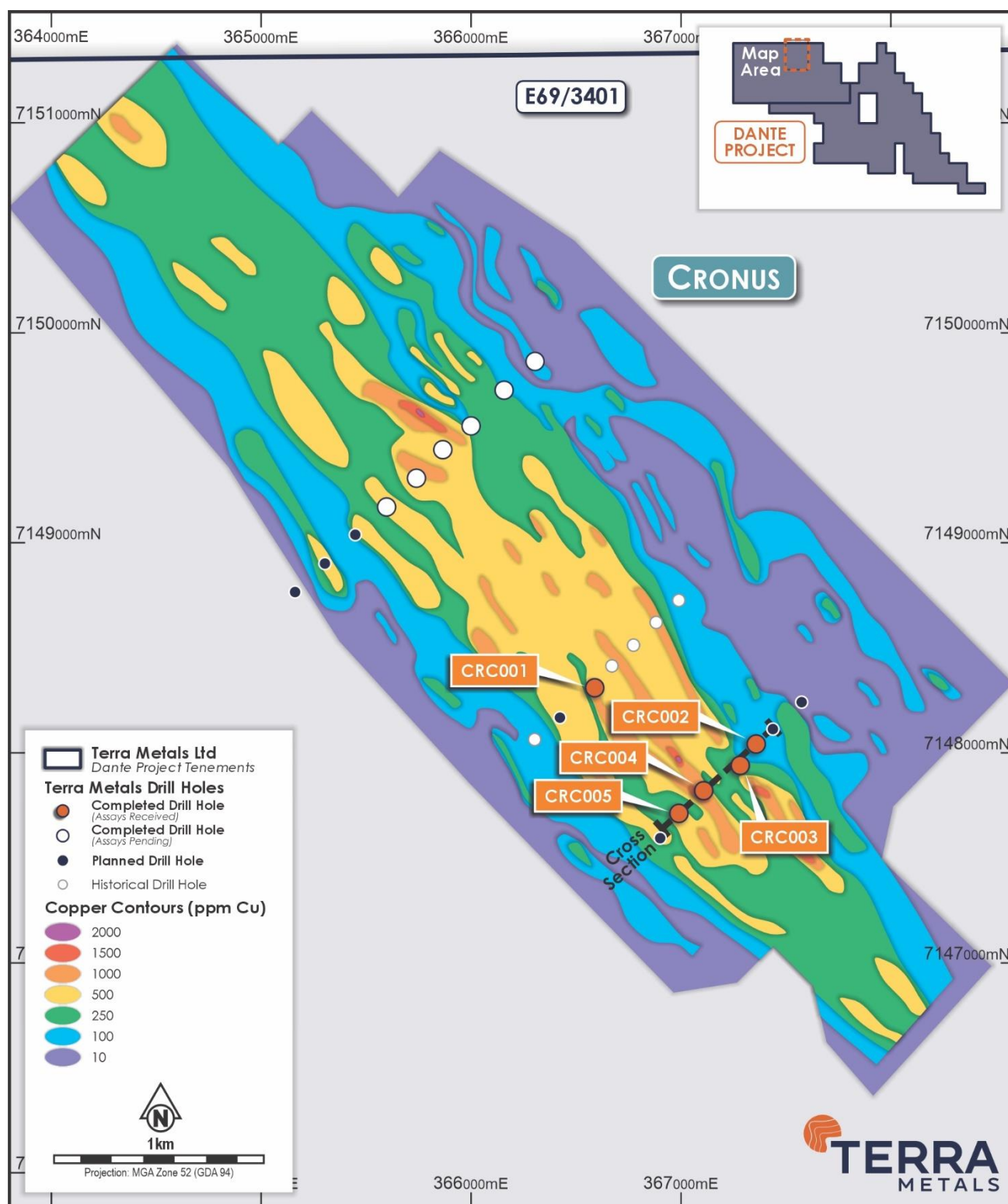
Figure 8. The Cronus Prospect copper auger geochemistry , showing current and historical drilling.
