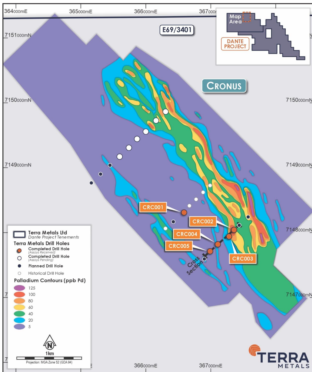
Figure 10. The Cronus Prospect palladium auger geochemistry , showing current and historical drilling.
