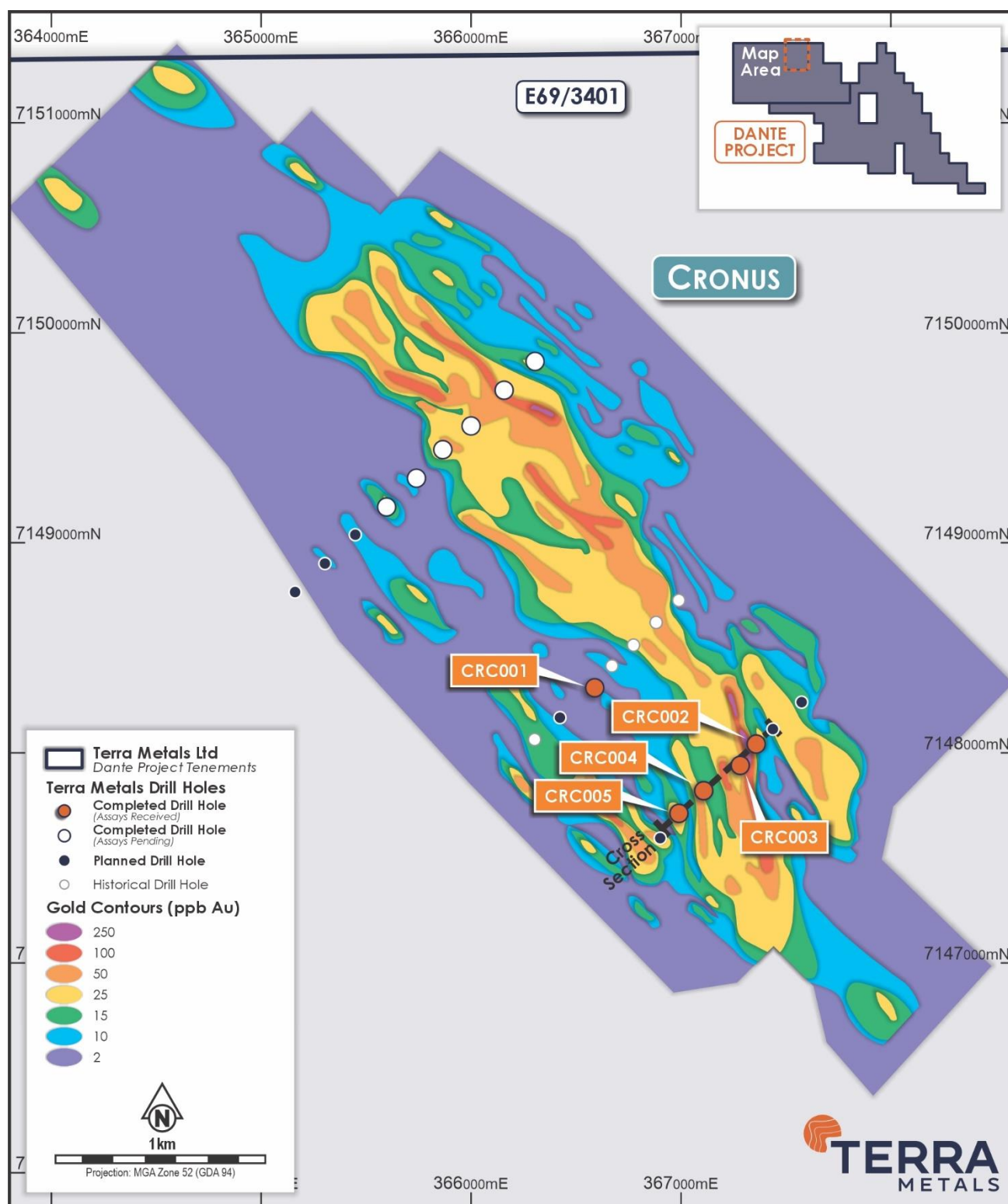
Figure 9. The Cronus Prospect gold auger geochemistry , showing current and historical drilling.
