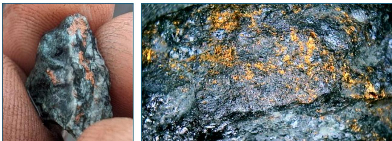
Figure 6. Examples of (left) Native Copper development (scale 2cm) in upper gabbronorite hanging wall; and (right) copper-sulphides (scale 1cm) in the basal Crius Reef
