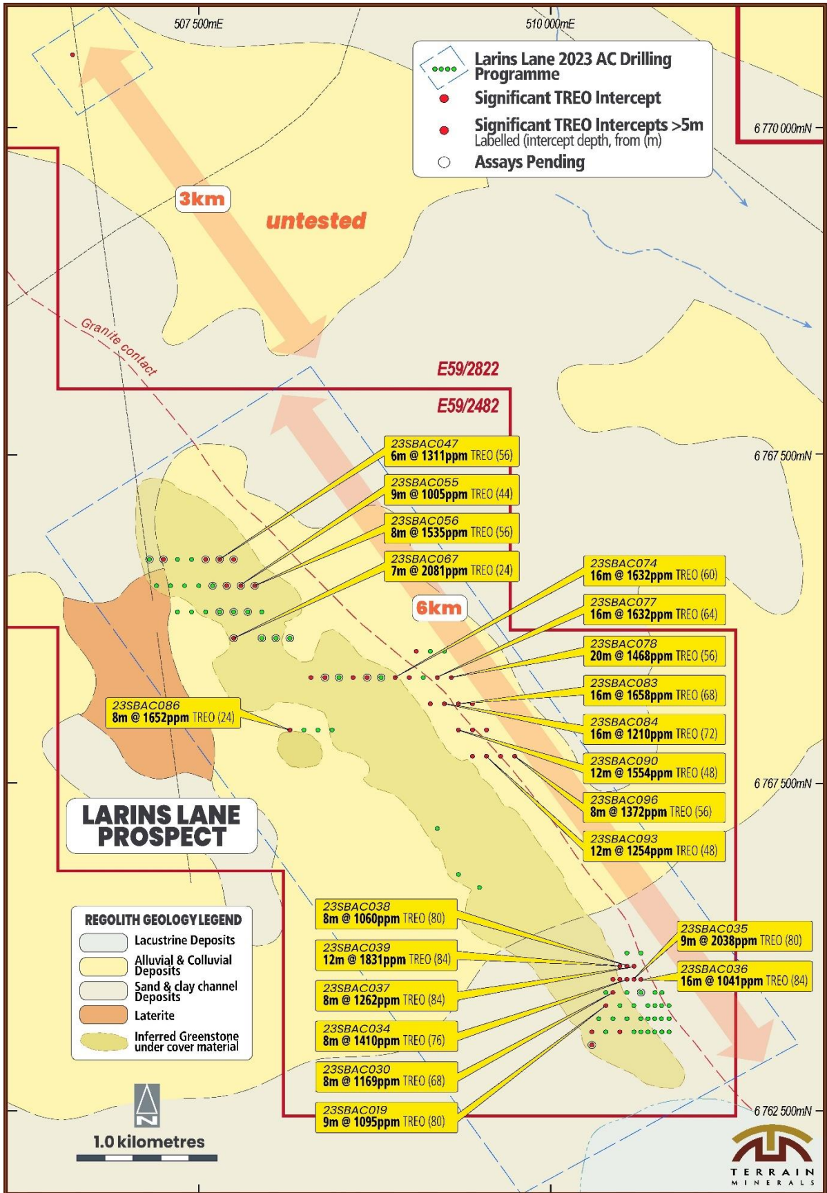
Diagram 1: Drill hole location of Terrain’s 2023 air core drill program at the Larins Lane Project with selected total rare earth oxide (TREO) grades highlighted. Intercepts are based on 1,000ppm TREO lower cut and up to four metres internal dilution. A significant TREO intercept, as referred to in this diagram, is an interval returning greater than 1,000ppm TREO over a minimum of one composite sample (generally being three or four metres).
