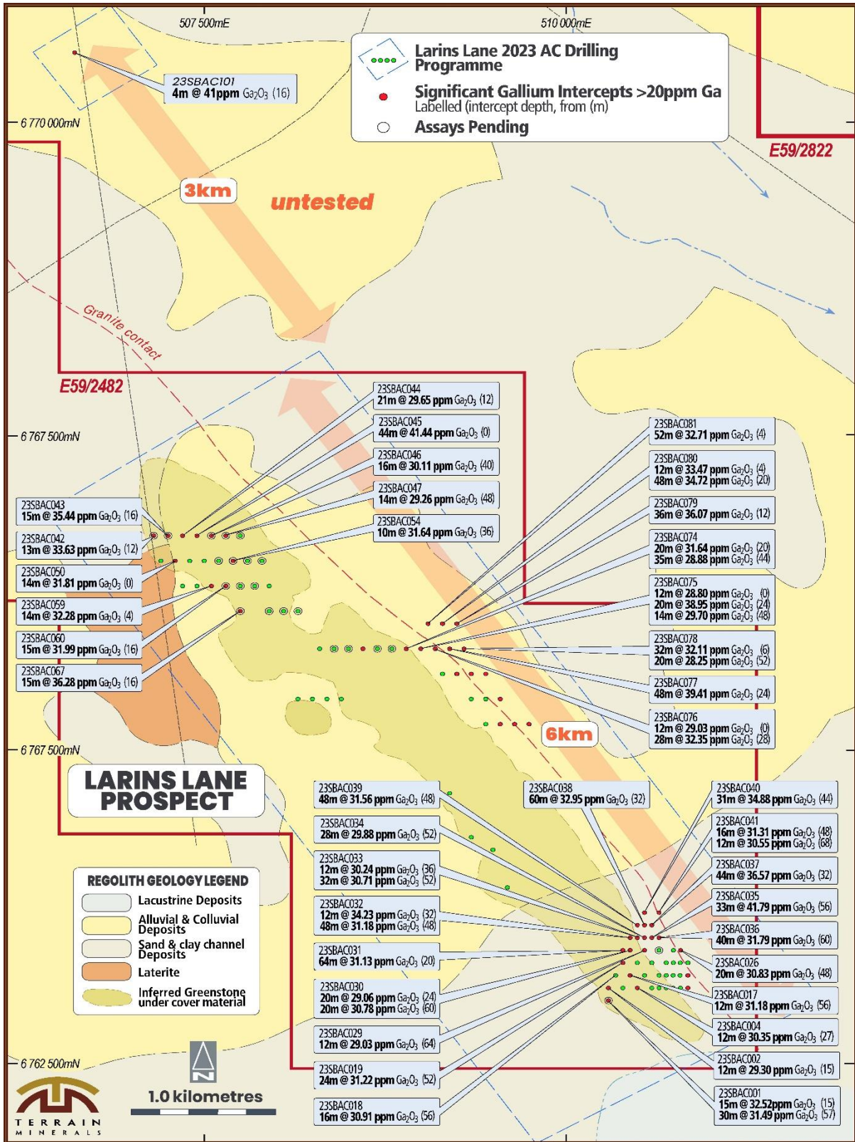
Diagram 2: Drill hole location (Not possible to show all) of Terrain’s 2023 air core drill program at the Larins Lane Project with selected gallium oxide grades highlighted. Intercepts are based on 20ppm gallium (26.88ppm Ga 2 O 3 ) lower cut and up to four metres internal dilution. A significant gallium oxide intercept, as referred to in this diagram, is an interval returning greater than 20ppm gallium (26.88ppm Ga 2 O 3 ) lower cut over a minimum of one composite sample (generally being three or four metres).
