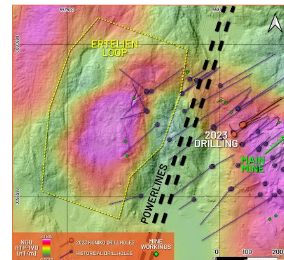
Ertelien Ground Electromagnetic Survey Targets
