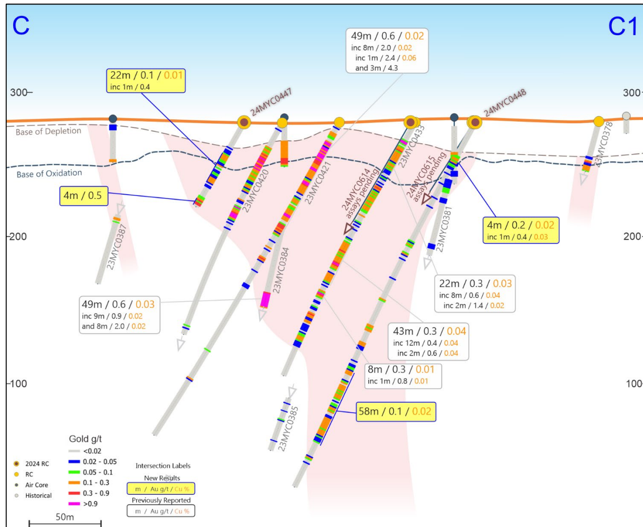
Figure 6: GEO-01 deposit NW-SE cross-section C-C1 (refer to Figure 3 for location) showing gold±copper drill intercepts, with the deposit open down dip and along strike for multiple zones of mineralisation. NB: 100m elevation (RL), looking toward 035° GDA2020 / MGA Zone 51 Grid.
