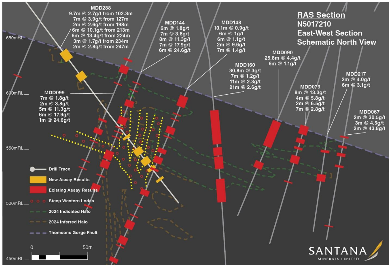
Figure 2 Cross Section N5017210 illustrating the steep western lodes encountered in MDD288.
