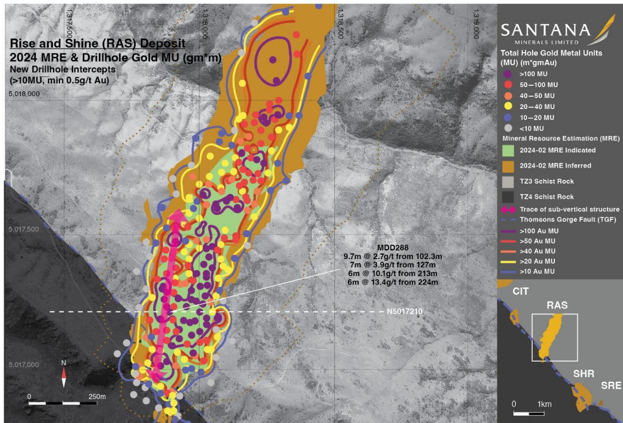
Figure 1 Plan view of RAS with MDD288 and sub-vertical steep western lodes (pink arrow) in RAS Deposit.
