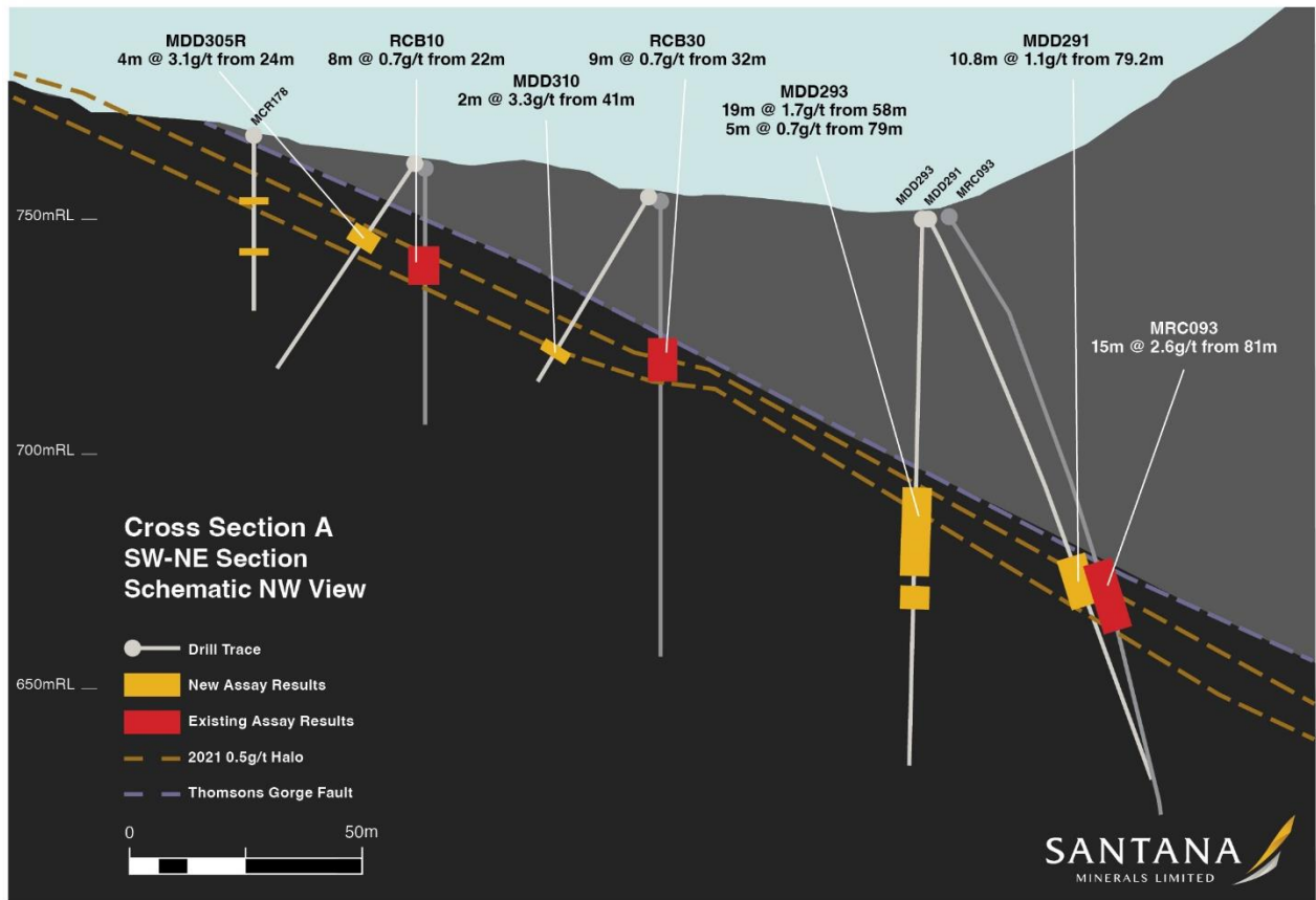
Figure 4 Cross Section A, showing new assays in orange and existing assays in red, along with inferred halo boundaries.
