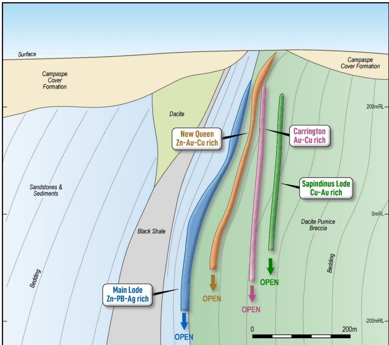
Figure 4: Schematic cross section (looking west) of the various lodes at Liontown West. Highlighted are the stratigraphy parallel Main (blue) and New Queen (orange) Lodes and the sub-vertical Carrington (pink) and Sapindinus (green) Lodes.
