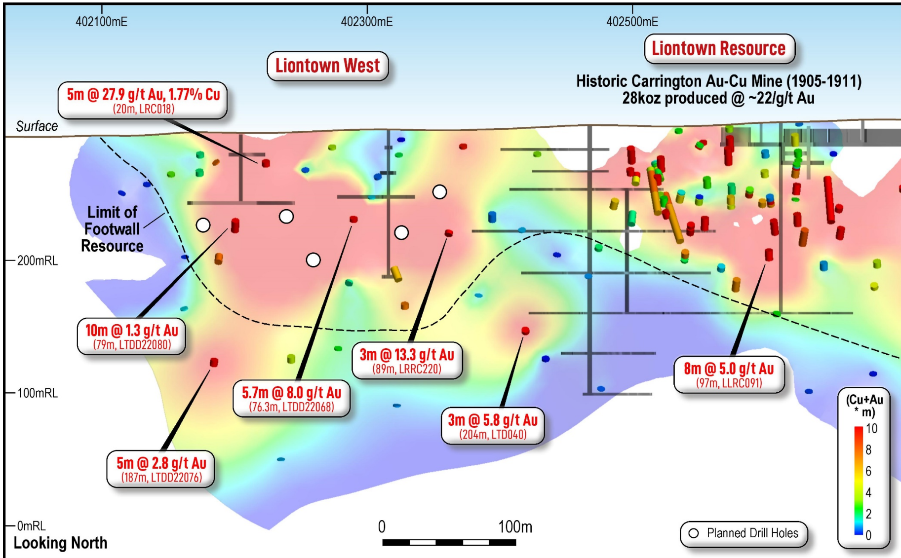
Figure 3: Long section (20m thick) of the Au-Cu rich footwall horizon at Liontown West, coloured by thickness. Key historic intercepts, historic workings including the Carrington Au-Cu Mine and planned infill RC holes (white dots) are displayed.
