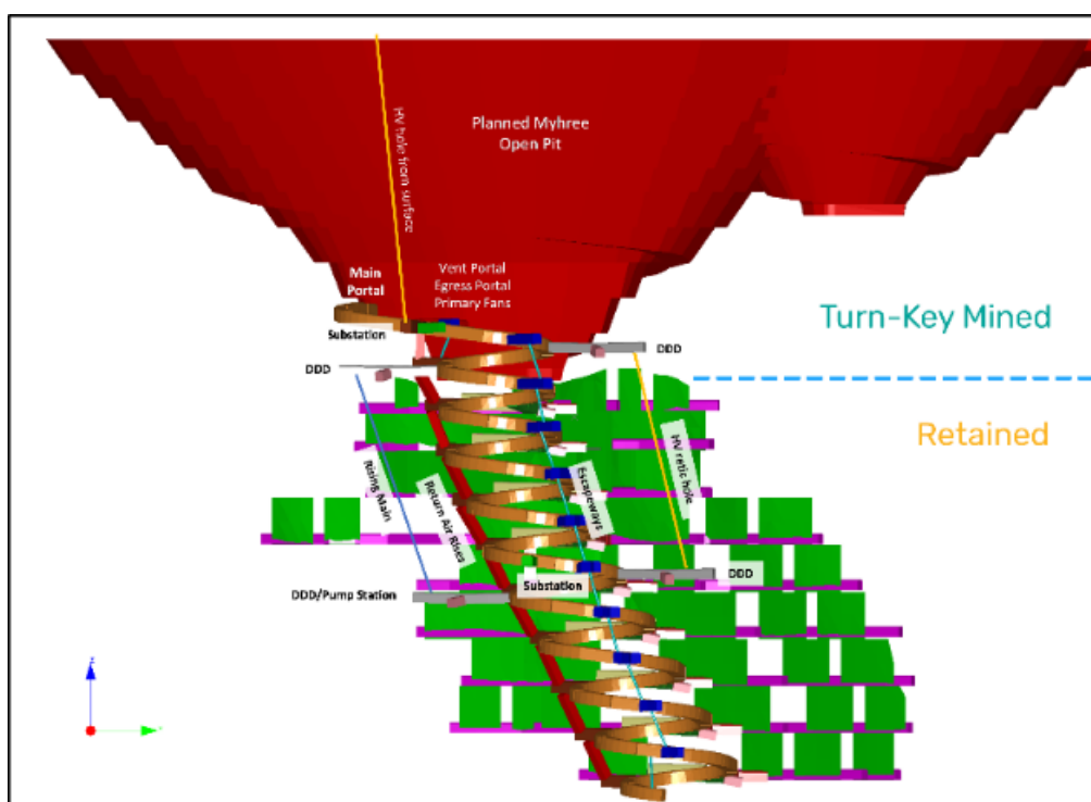
Figure 6: Long section view (looking west) of the planned Myhree open pit, and the planned underground mine retained by Black Cat
