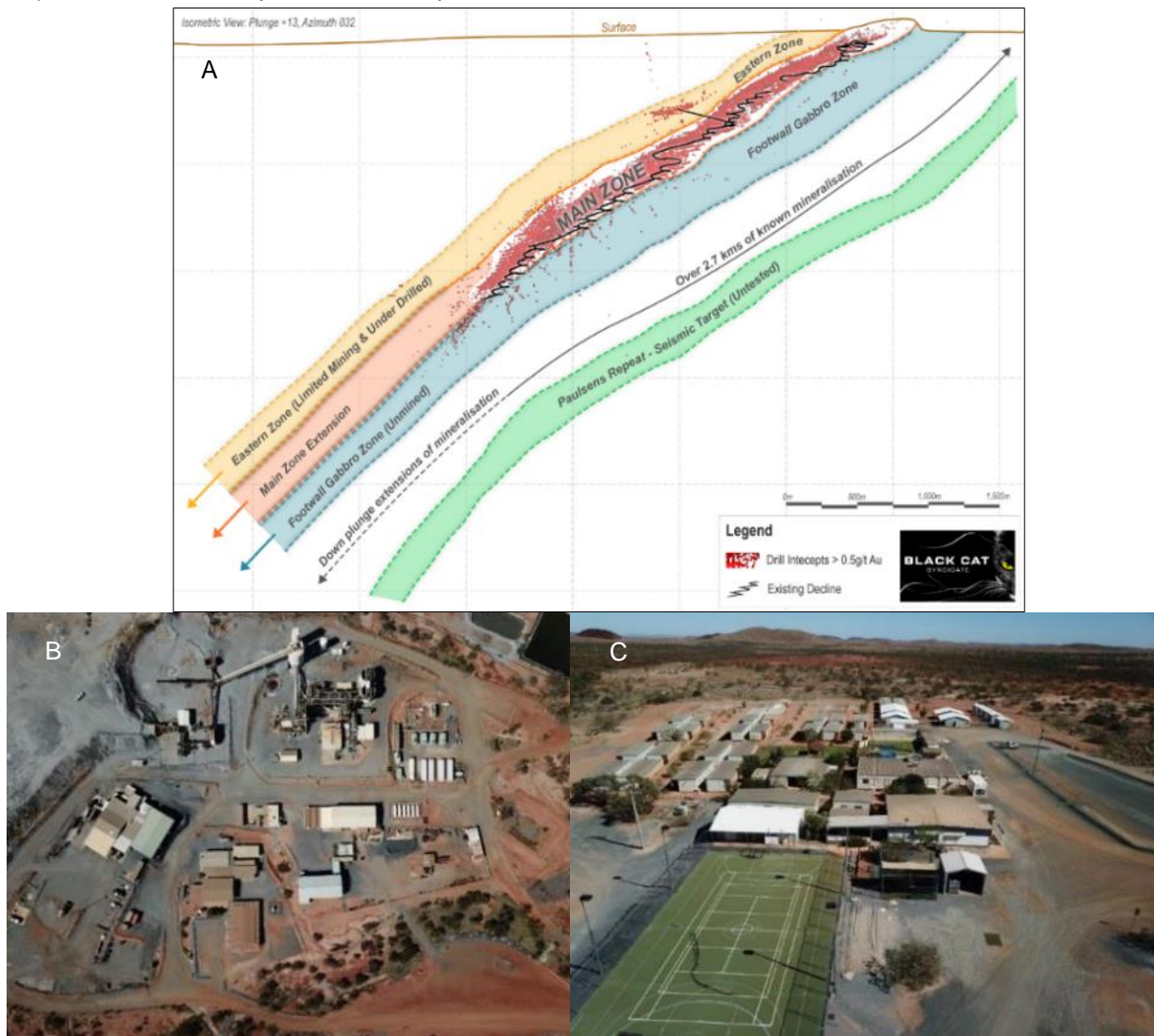
Figure 2A. Schematic isometric long-section looking towards the north showing >2.7km of known mineralisation comprised of: Main Zone (~1Moz mined @ 1,000oz per vertical metre), under-drilled Eastern Zone, unmined Footwall Gabbro Zone and the Paulsens Repeat seismic target; 2B. Aerial view of Paulsens processing facility and site offices; and 2C. Paulsens village and camp
